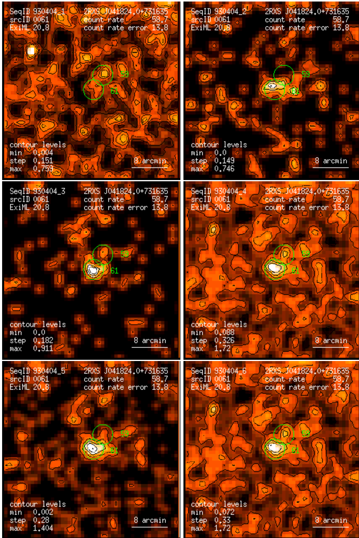
Figure 61: RASS 930404: detection 0061: band rate images, Gaussian filter: (1) PSPC channels 11 – 41, (2) 52 – 90, (3) 91 – 201, (4) 11 – 235, (5) 52 – 201, (6) 11 – 201. Broad band rates in counts/ks. Band rate contour levels in counts/ks/arcmin 2 .
