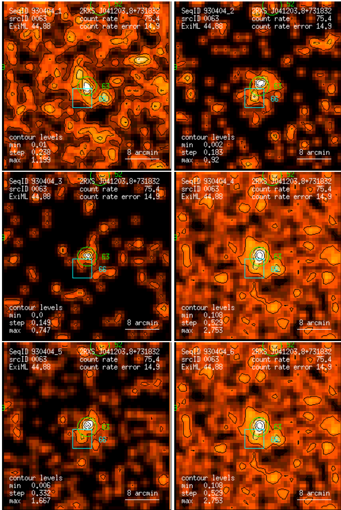
Figure 63: RASS 930404: detection 0063: band rate images, Gaussian filter: (1) PSPC channels 11 – 41, (2) 52 – 90, (3) 91 – 201, (4) 11 – 235, (5) 52 – 201, (6) 11 – 201. Broad band rates in counts/ks. Band rate contour levels in counts/ks/arcmin 2 .
