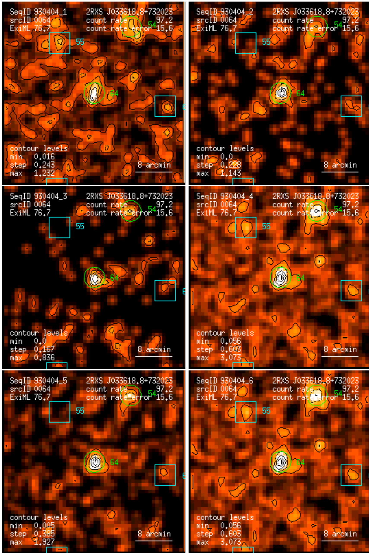
Figure 64: RASS 930404: detection 0064: band rate images, Gaussian filter: (1) PSPC channels 11 – 41, (2) 52 – 90, (3) 91 – 201, (4) 11 – 235, (5) 52 – 201, (6) 11 – 201. Broad band rates in counts/ks. Band rate contour levels in counts/ks/arcmin 2 .
