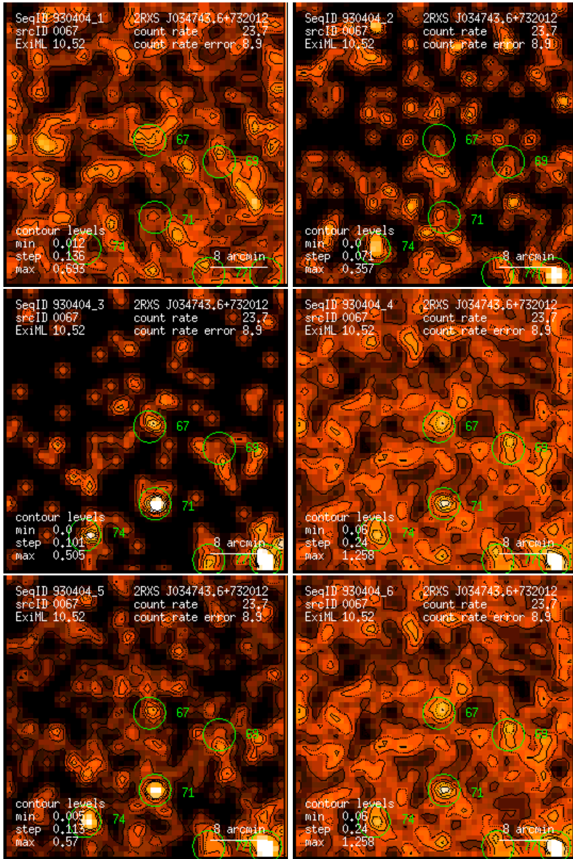
Figure 67: RASS 930404: detection 0067: band rate images, Gaussian filter: (1) PSPC channels 11 – 41, (2) 52 – 90, (3) 91 – 201, (4) 11 – 235, (5) 52 – 201, (6) 11 – 201. Broad band rates in counts/ks. Band rate contour levels in counts/ks/arcmin 2 .
