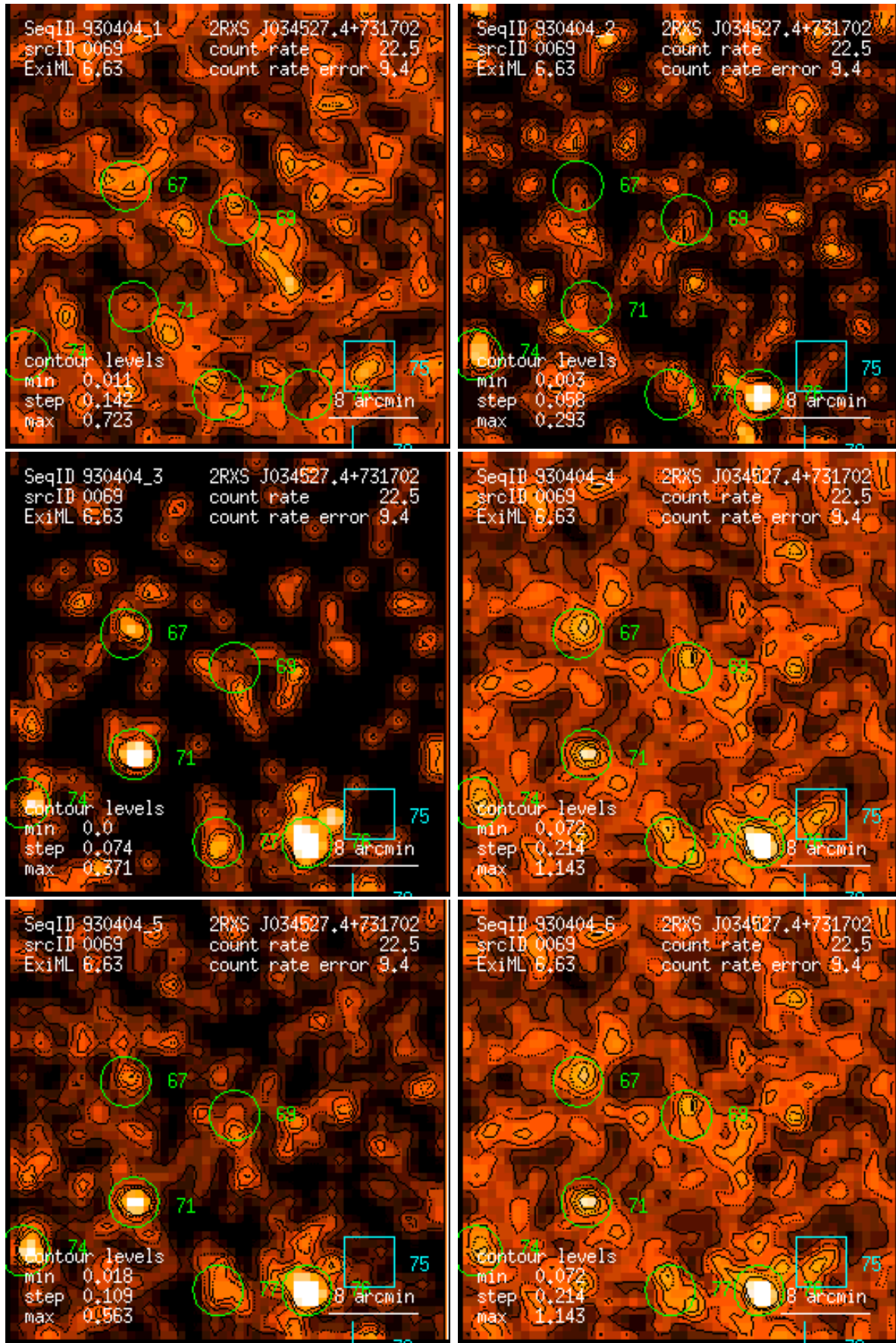
Figure 69: RASS 930404: detection 0069: band rate images, Gaussian filter: (1) PSPC channels 11 – 41, (2) 52 – 90, (3) 91 – 201, (4) 11 – 235, (5) 52 – 201, (6) 11 – 201. Broad band rates in counts/ks. Band rate contour levels in counts/ks/arcmin 2 .
