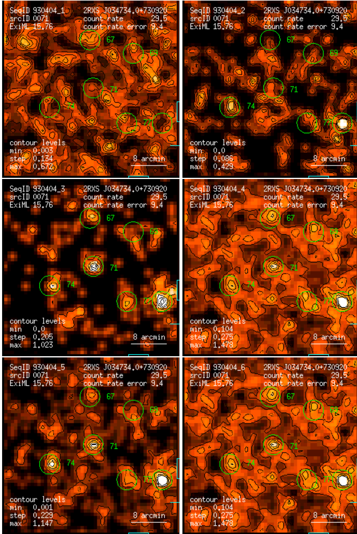
Figure 71: RASS 930404: detection 0071: band rate images, Gaussian filter: (1) PSPC channels 11 – 41, (2) 52 – 90, (3) 91 – 201, (4) 11 – 235, (5) 52 – 201, (6) 11 – 201. Broad band rates in counts/ks. Band rate contour levels in counts/ks/arcmin 2 .
