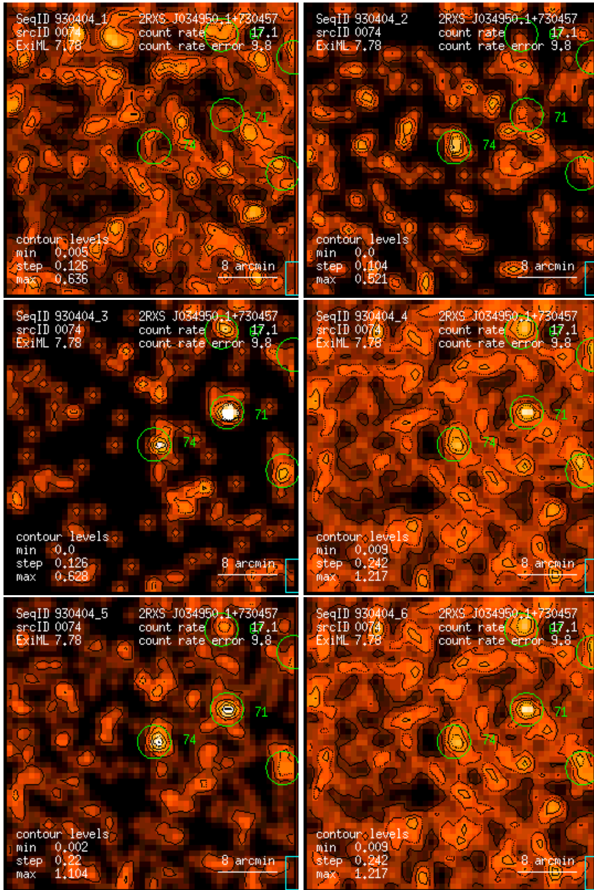
Figure 74: RASS 930404: detection 0074: band rate images, Gaussian filter: (1) PSPC channels 11 – 41, (2) 52 – 90, (3) 91 – 201, (4) 11 – 235, (5) 52 – 201, (6) 11 – 201. Broad band rates in counts/ks. Band rate contour levels in counts/ks/arcmin 2 .
