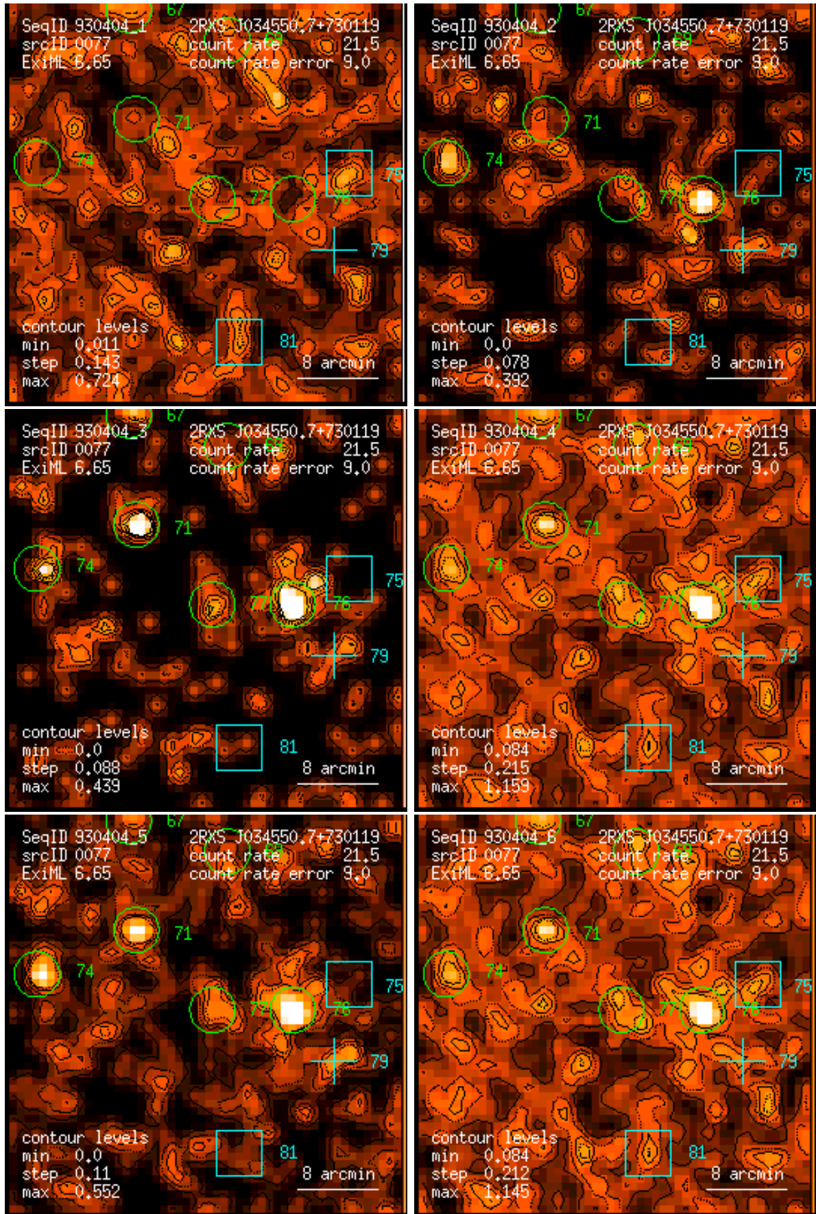
Figure 77: RASS 930404: detection 0077: band rate images, Gaussian filter: (1) PSPC channels 11 – 41, (2) 52 – 90, (3) 91 – 201, (4) 11 – 235, (5) 52 – 201, (6) 11 – 201. Broad band rates in counts/ks. Band rate contour levels in counts/ks/arcmin 2 .
