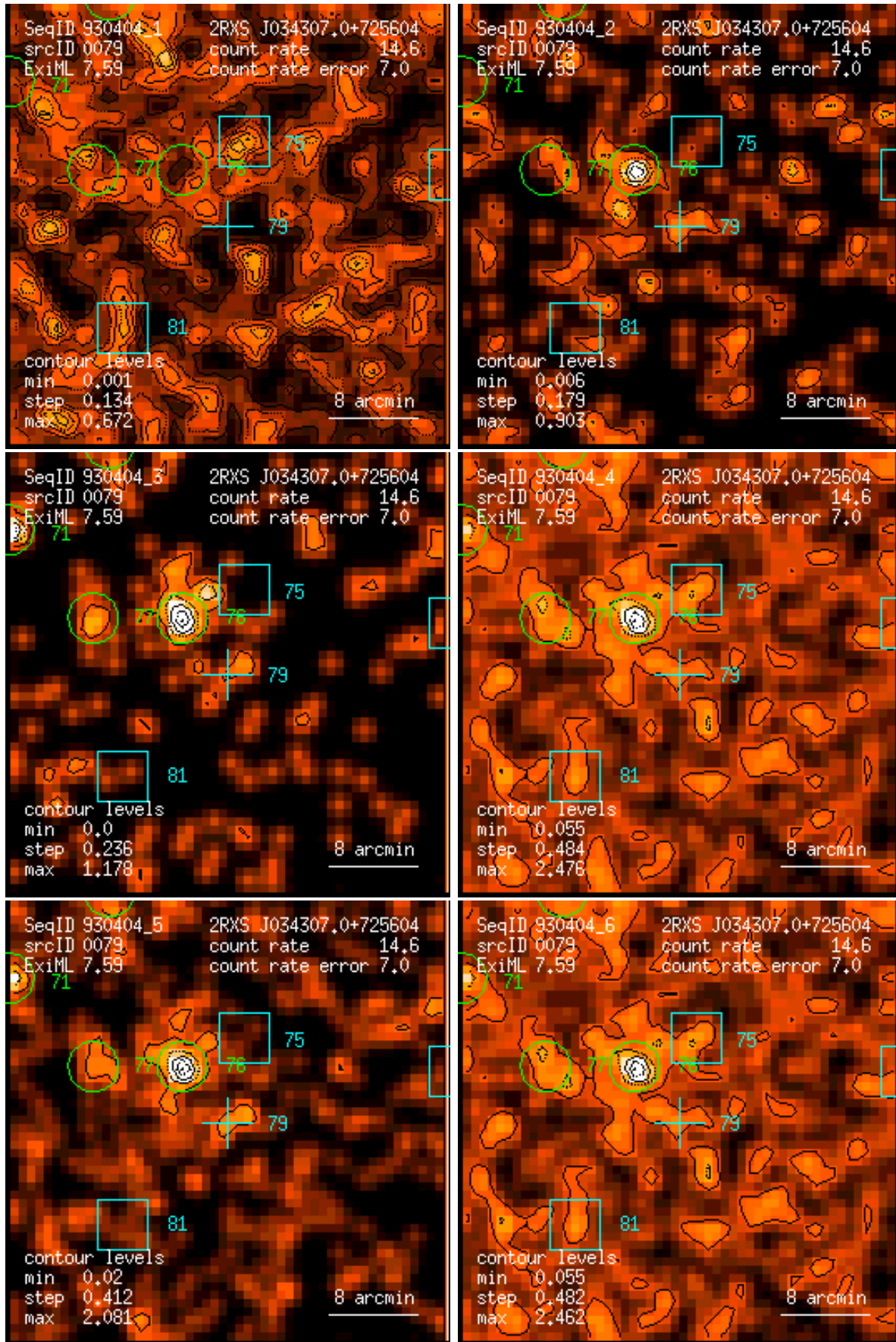
Figure 79: RASS 930404: detection 0079: band rate images, Gaussian filter: (1) PSPC channels 11 – 41, (2) 52 – 90, (3) 91 – 201, (4) 11 – 235, (5) 52 – 201, (6) 11 – 201. Broad band rates in counts/ks. Band rate contour levels in counts/ks/arcmin 2 .
