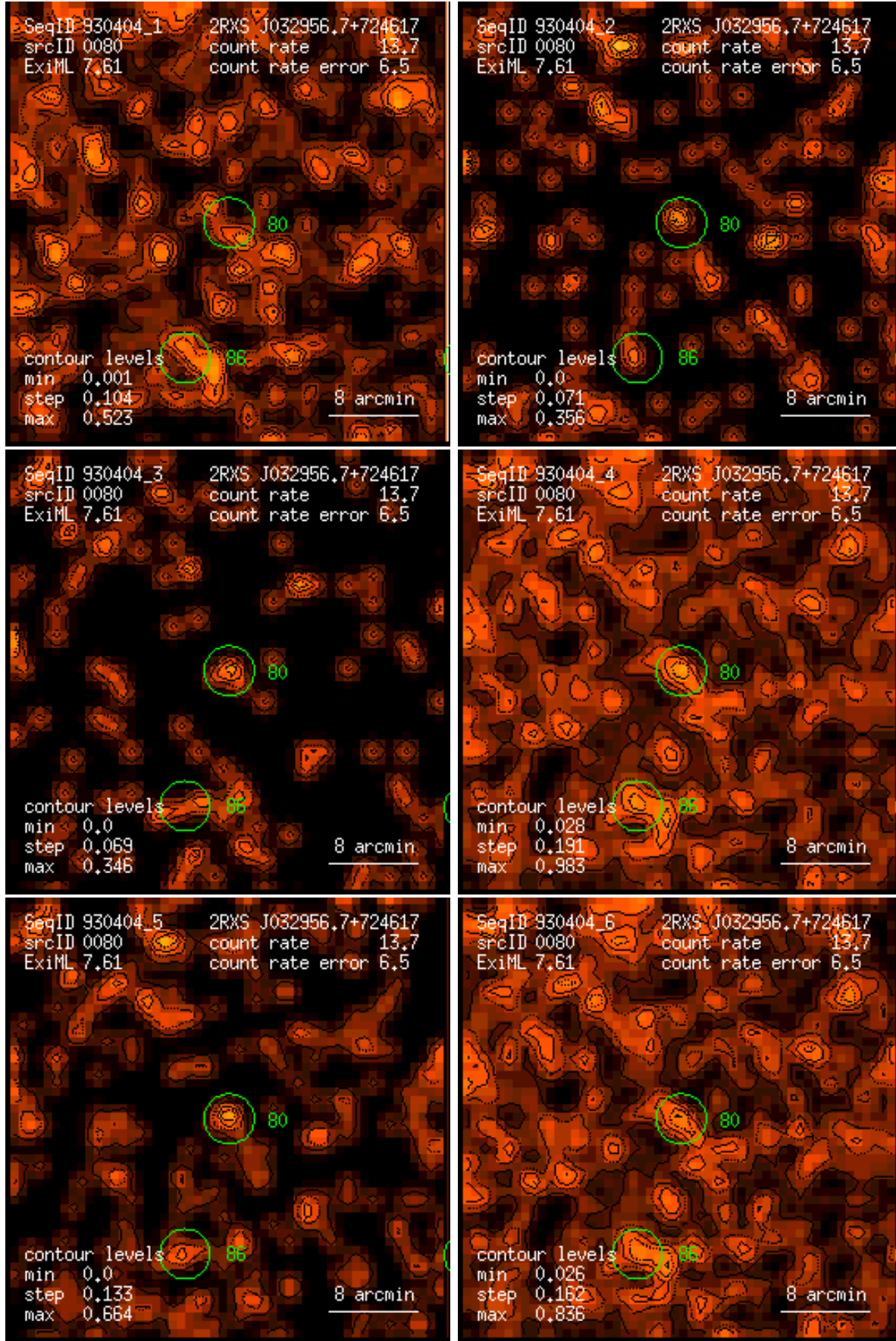
Figure 80: RASS 930404: detection 0080: band rate images, Gaussian filter: (1) PSPC channels 11 – 41, (2) 52 – 90, (3) 91 – 201, (4) 11 – 235, (5) 52 – 201, (6) 11 – 201. Broad band rates in counts/ks. Band rate contour levels in counts/ks/arcmin 2 .
