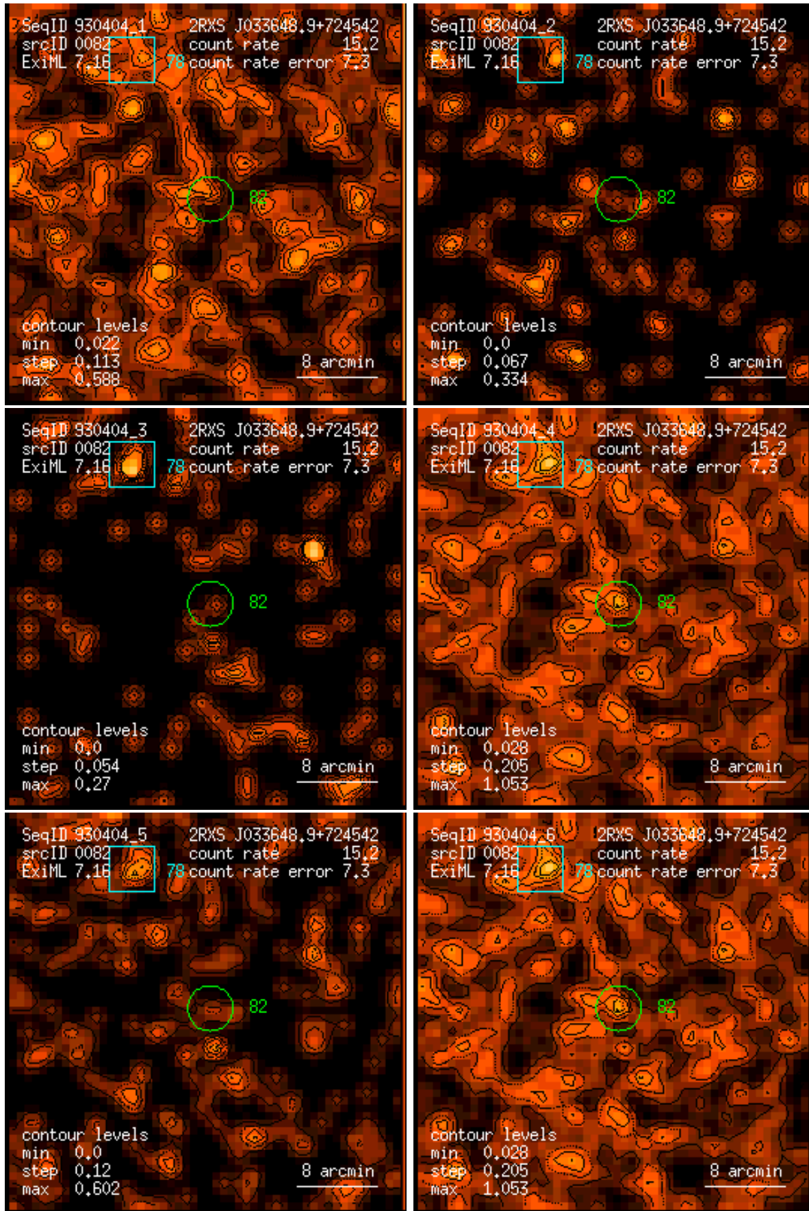
Figure 82: RASS 930404: detection 0082: band rate images, Gaussian filter: (1) PSPC channels 11 – 41, (2) 52 – 90, (3) 91 – 201, (4) 11 – 235, (5) 52 – 201, (6) 11 – 201. Broad band rates in counts/ks. Band rate contour levels in counts/ks/arcmin 2 .
