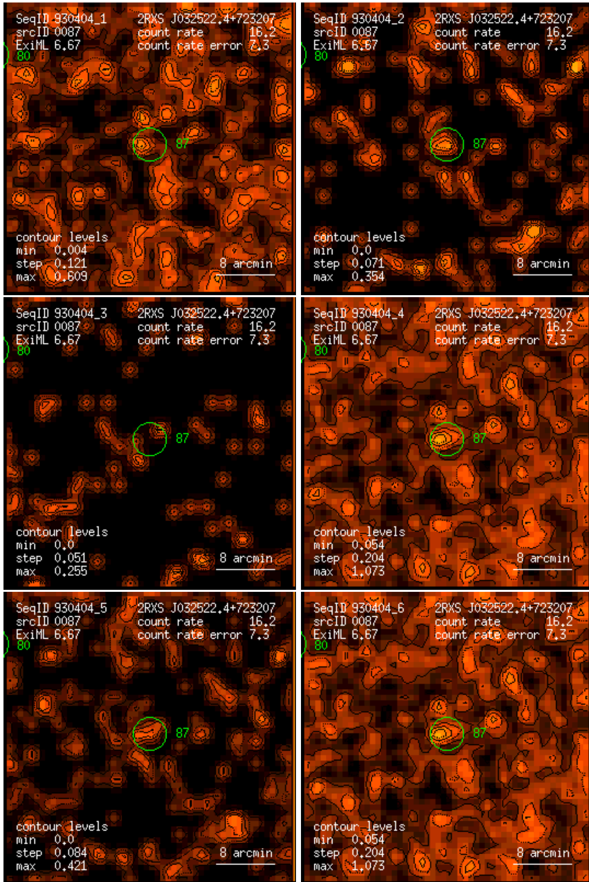
Figure 87: RASS 930404: detection 0087: band rate images, Gaussian filter: (1) PSPC channels 11 – 41, (2) 52 – 90, (3) 91 – 201, (4) 11 – 235, (5) 52 – 201, (6) 11 – 201. Broad band rates in counts/ks. Band rate contour levels in counts/ks/arcmin 2 .
