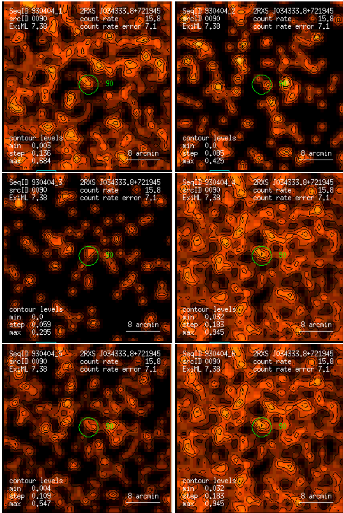
Figure 90: RASS 930404: detection 0090: band rate images, Gaussian filter: (1) PSPC channels 11 – 41, (2) 52 – 90, (3) 91 – 201, (4) 11 – 235, (5) 52 – 201, (6) 11 – 201. Broad band rates in counts/ks. Band rate contour levels in counts/ks/arcmin 2 .
