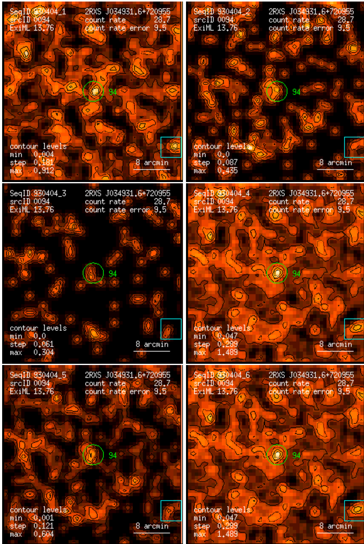
Figure 94: RASS 930404: detection 0094: band rate images, Gaussian filter: (1) PSPC channels 11 – 41, (2) 52 – 90, (3) 91 – 201, (4) 11 – 235, (5) 52 – 201, (6) 11 – 201. Broad band rates in counts/ks. Band rate contour levels in counts/ks/arcmin 2 .
