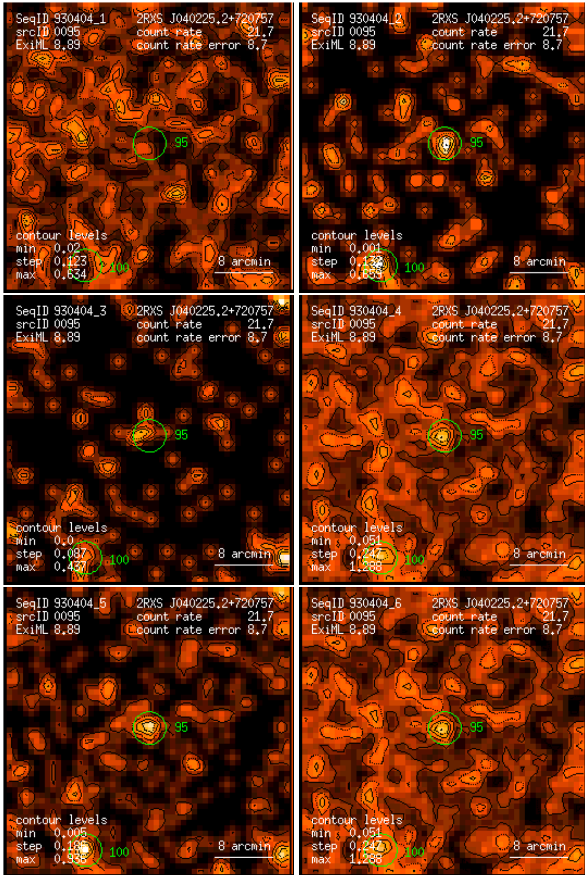
Figure 95: RASS 930404: detection 0095: band rate images, Gaussian filter: (1) PSPC channels 11 – 41, (2) 52 – 90, (3) 91 – 201, (4) 11 – 235, (5) 52 – 201, (6) 11 – 201. Broad band rates in counts/ks. Band rate contour levels in counts/ks/arcmin 2 .
