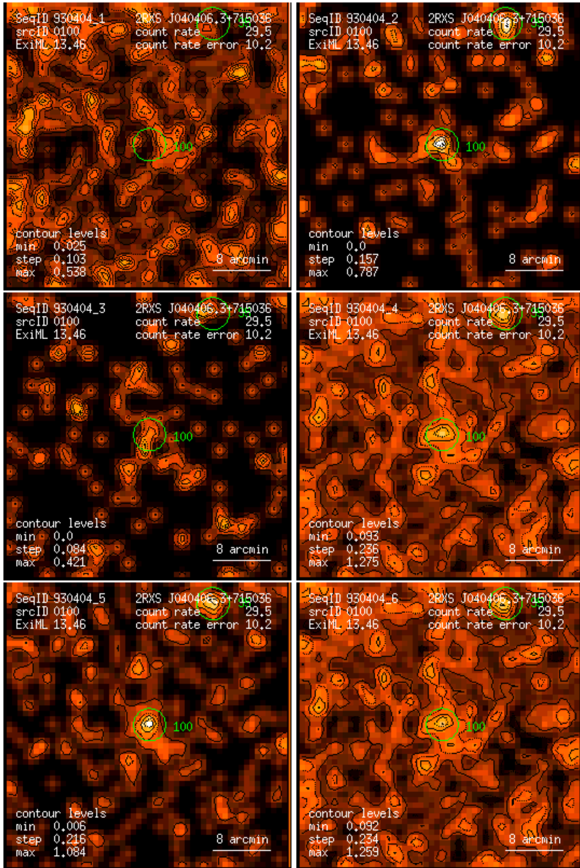
Figure 100: RASS 930404: detection 0100: band rate images, Gaussian filter: (1) PSPC channels 11 – 41, (2) 52 – 90, (3) 91 – 201, (4) 11 – 235, (5) 52 – 201, (6) 11 – 201. Broad band rates in counts/ks. Band rate contour levels in counts/ks/arcmin 2 .
