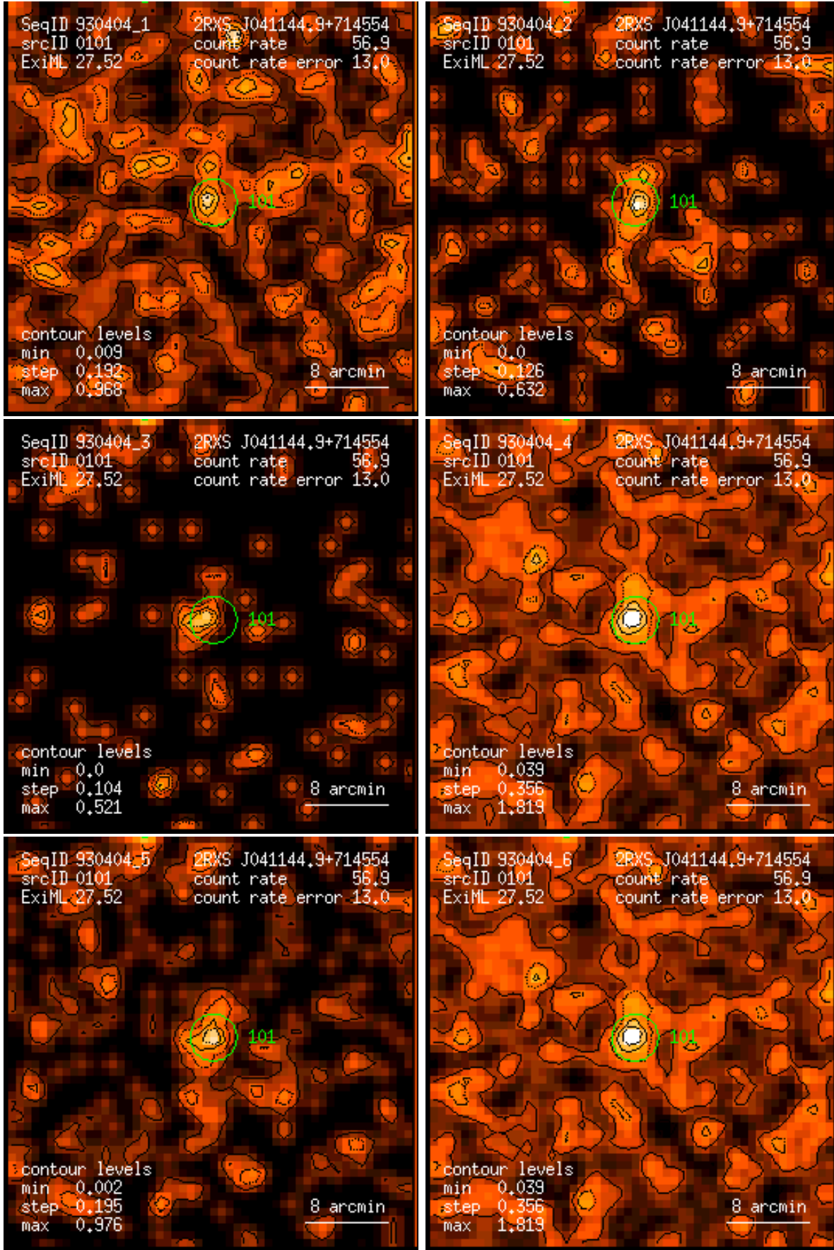
Figure 101: RASS 930404: detection 0101: band rate images, Gaussian filter: (1) PSPC channels 11 – 41, (2) 52 – 90, (3) 91 – 201, (4) 11 – 235, (5) 52 – 201, (6) 11 – 201. Broad band rates in counts/ks. Band rate contour levels in counts/ks/arcmin 2 .
