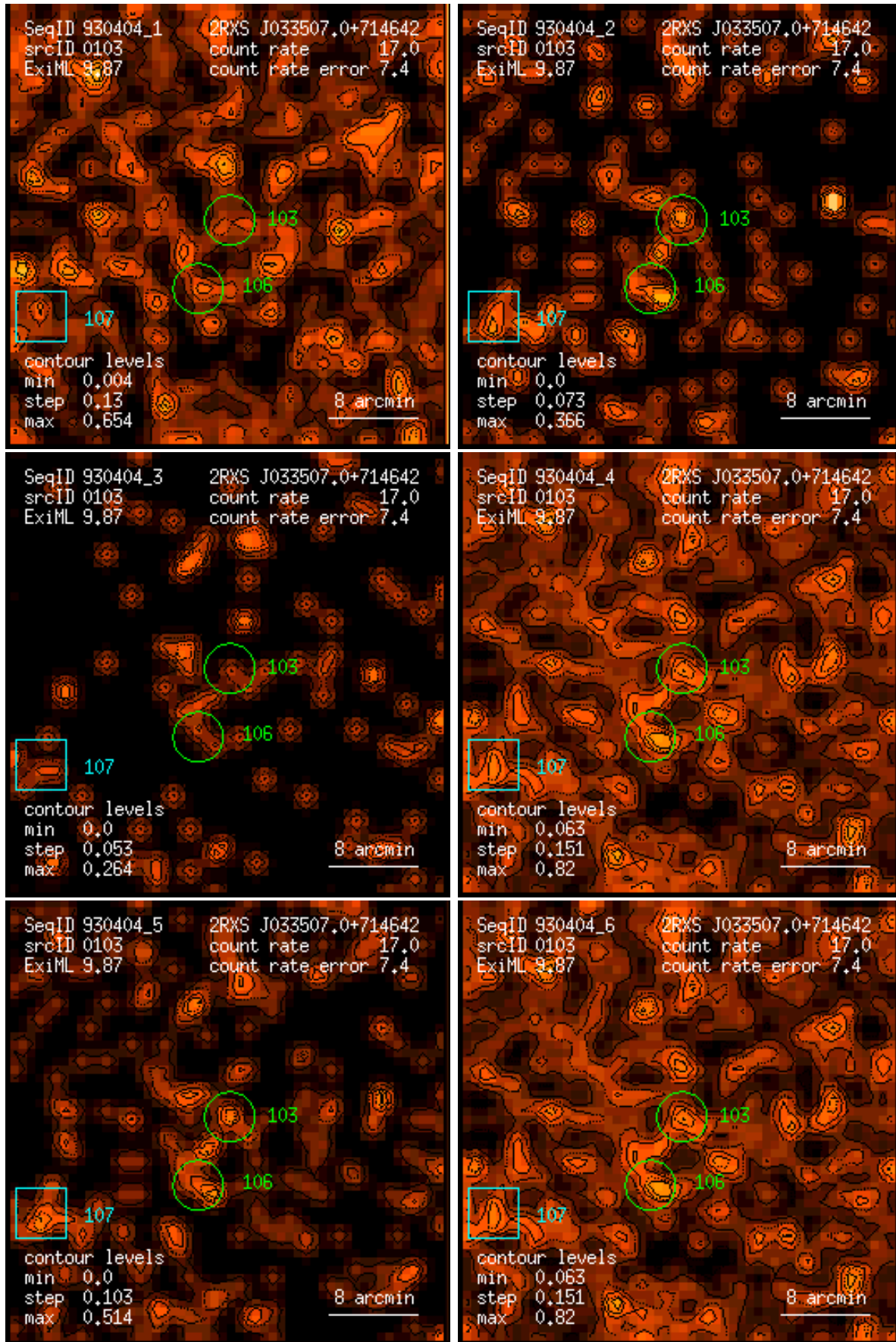
Figure 103: RASS 930404: detection 0103: band rate images, Gaussian filter: (1) PSPC channels 11 – 41, (2) 52 – 90, (3) 91 – 201, (4) 11 – 235, (5) 52 – 201, (6) 11 – 201. Broad band rates in counts/ks. Band rate contour levels in counts/ks/arcmin 2 .
