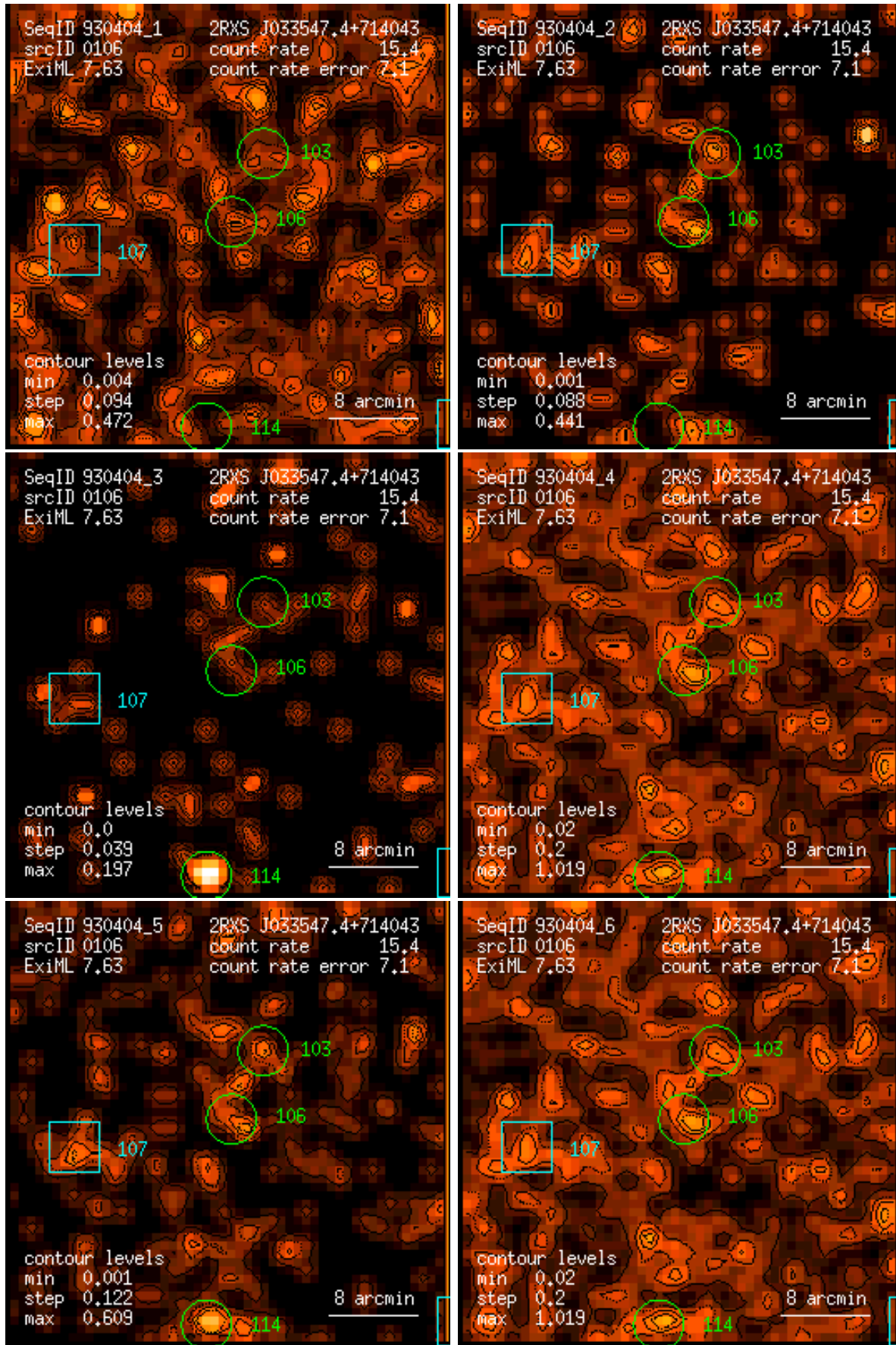
Figure 106: RASS 930404: detection 0106: band rate images, Gaussian filter: (1) PSPC channels 11 – 41, (2) 52 – 90, (3) 91 – 201, (4) 11 – 235, (5) 52 – 201, (6) 11 – 201. Broad band rates in counts/ks. Band rate contour levels in counts/ks/arcmin 2 .
