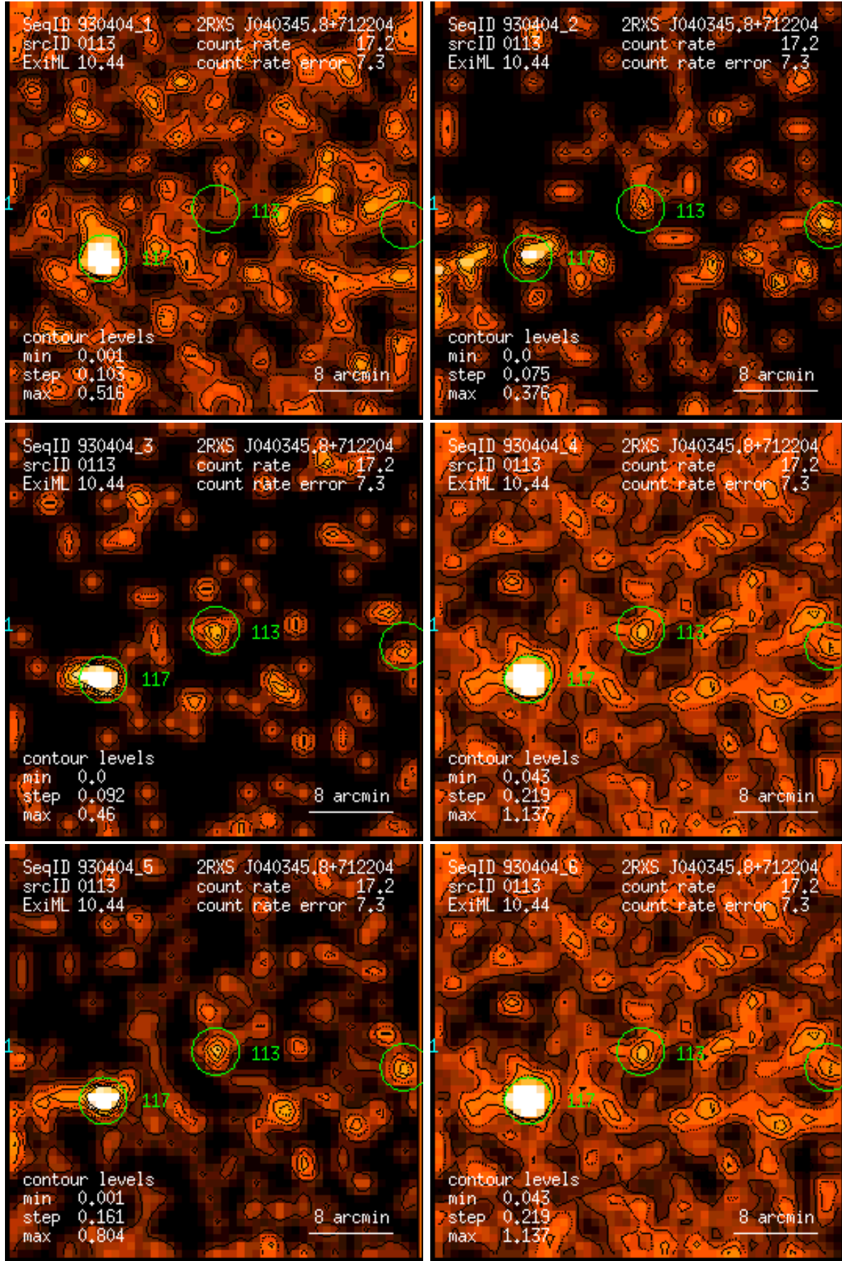
Figure 113: RASS 930404: detection 0113: band rate images, Gaussian filter: (1) PSPC channels 11 – 41, (2) 52 – 90, (3) 91 – 201, (4) 11 – 235, (5) 52 – 201, (6) 11 – 201. Broad band rates in counts/ks. Band rate contour levels in counts/ks/arcmin 2 .
