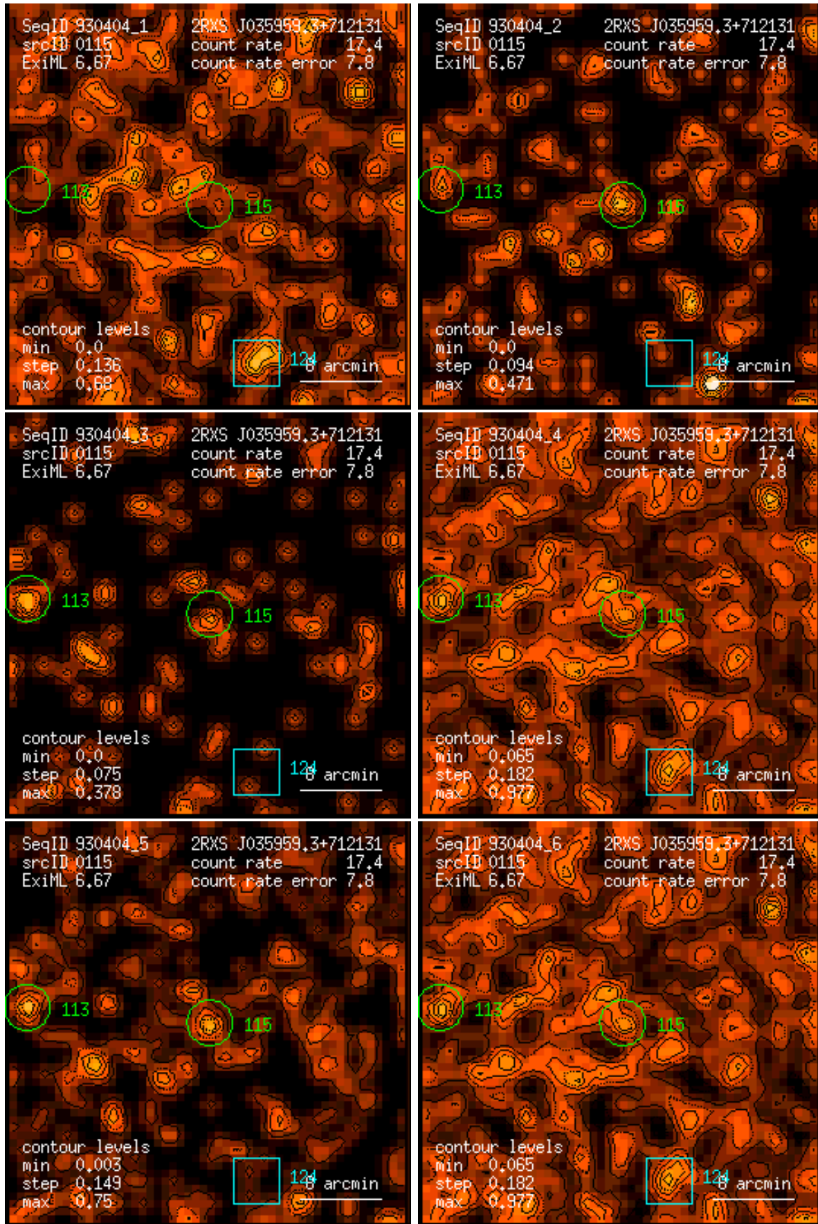
Figure 115: RASS 930404: detection 0115: band rate images, Gaussian filter: (1) PSPC channels 11 – 41, (2) 52 – 90, (3) 91 – 201, (4) 11 – 235, (5) 52 – 201, (6) 11 – 201. Broad band rates in counts/ks. Band rate contour levels in counts/ks/arcmin 2 .
