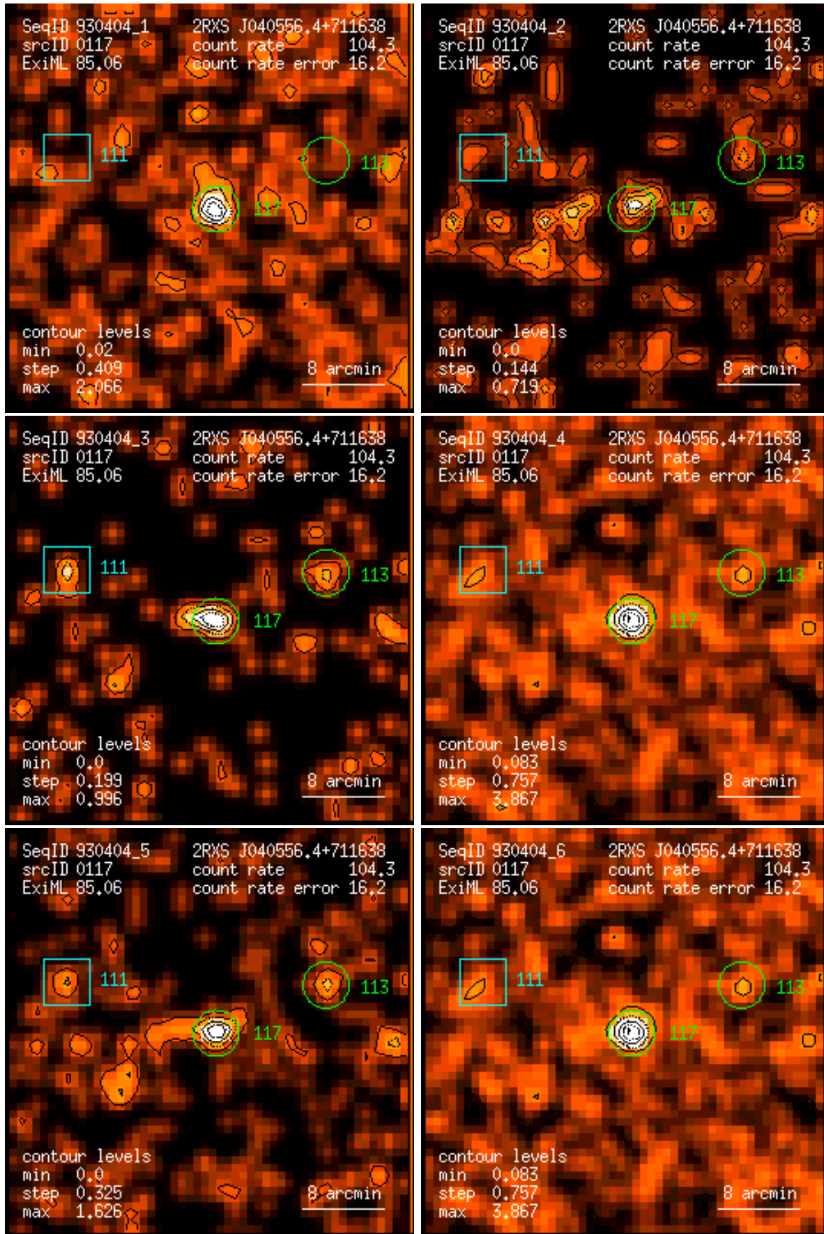
Figure 117: RASS 930404: detection 0117: band rate images, Gaussian filter: (1) PSPC channels 11 – 41, (2) 52 – 90, (3) 91 – 201, (4) 11 – 235, (5) 52 – 201, (6) 11 – 201. Broad band rates in counts/ks. Band rate contour levels in counts/ks/arcmin 2 .
