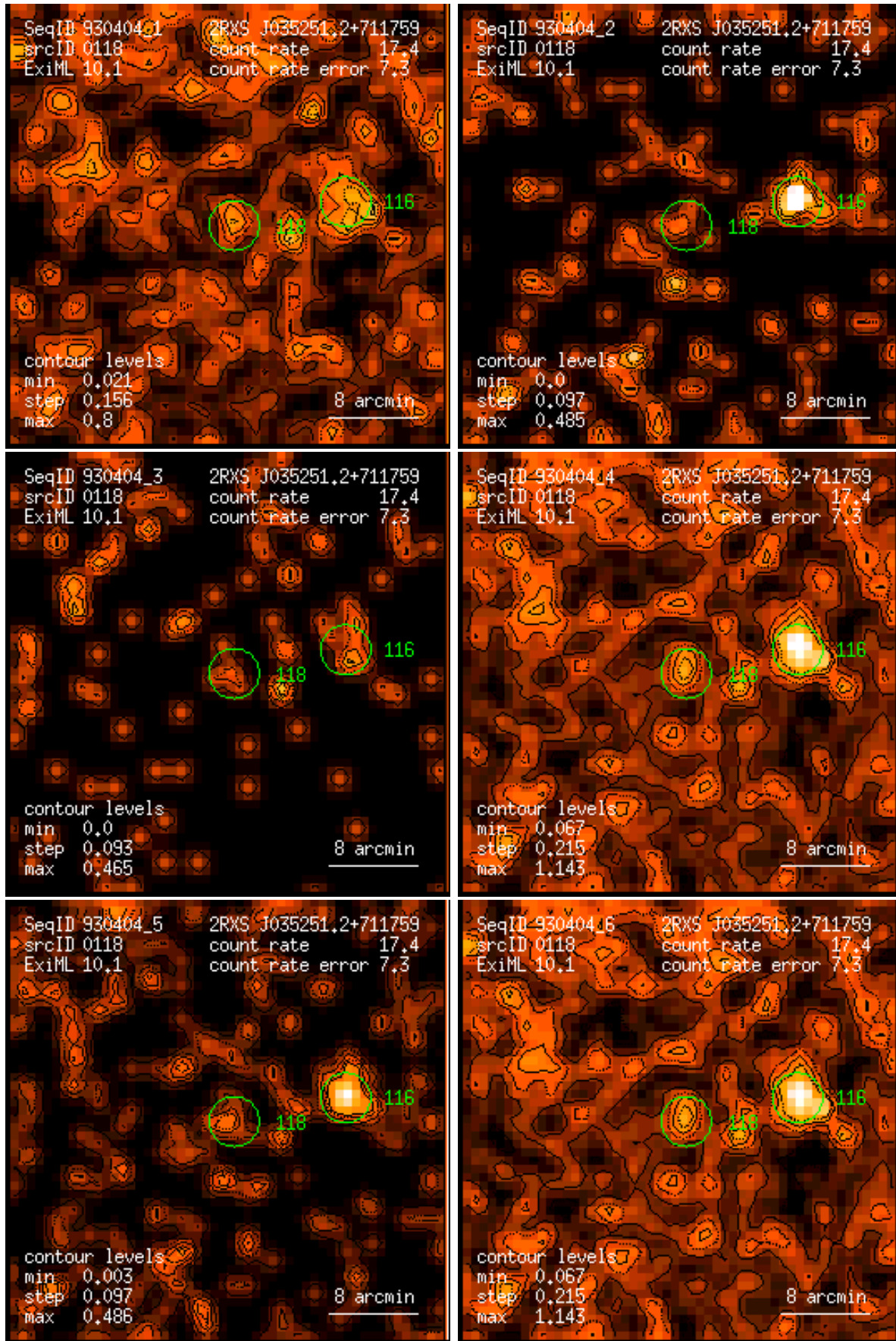
Figure 118: RASS 930404: detection 0118: band rate images, Gaussian filter: (1) PSPC channels 11 – 41, (2) 52 – 90, (3) 91 – 201, (4) 11 – 235, (5) 52 – 201, (6) 11 – 201. Broad band rates in counts/ks. Band rate contour levels in counts/ks/arcmin 2 .
