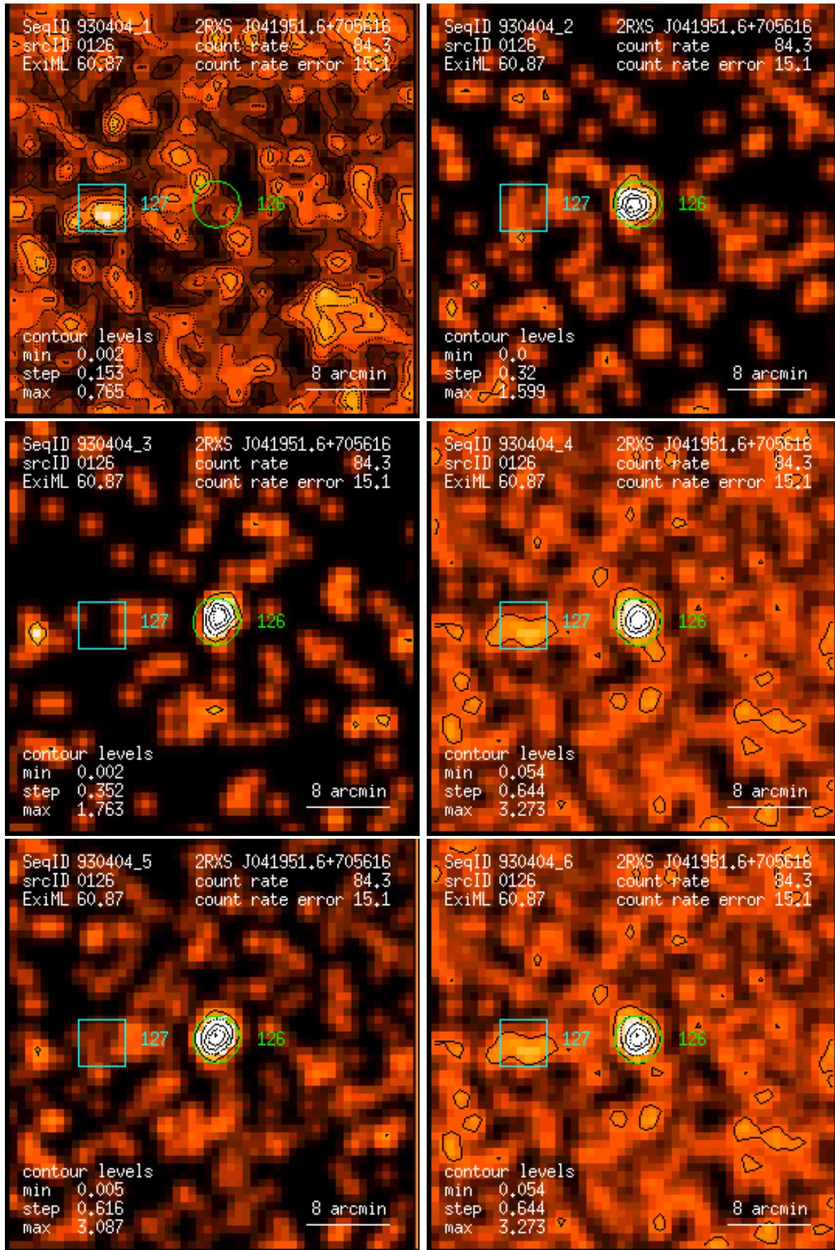
Figure 126: RASS 930404: detection 0126: band rate images, Gaussian filter: (1) PSPC channels 11 – 41, (2) 52 – 90, (3) 91 – 201, (4) 11 – 235, (5) 52 – 201, (6) 11 – 201. Broad band rates in counts/ks. Band rate contour levels in counts/ks/arcmin 2 .
