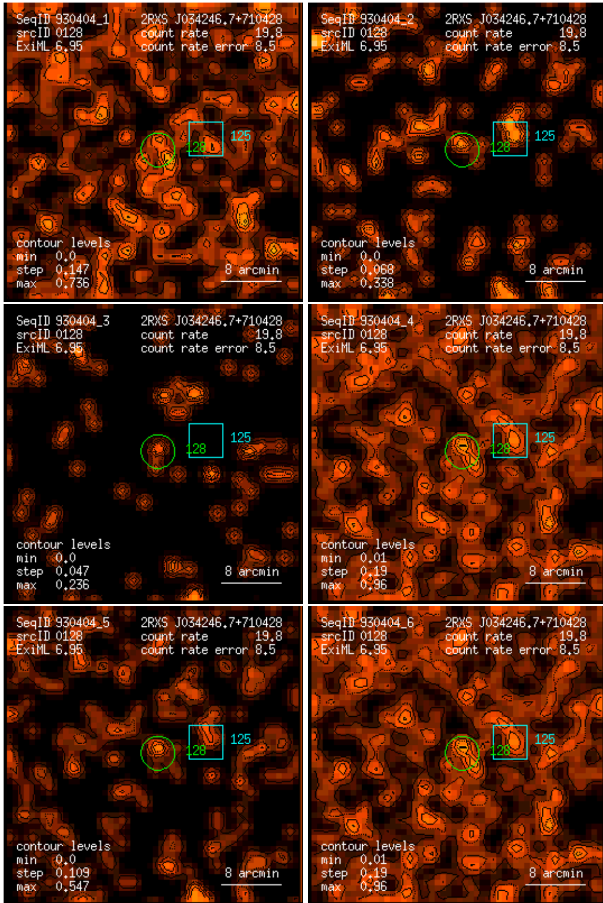
Figure 128: RASS 930404: detection 0128: band rate images, Gaussian filter: (1) PSPC channels 11 – 41, (2) 52 – 90, (3) 91 – 201, (4) 11 – 235, (5) 52 – 201, (6) 11 – 201. Broad band rates in counts/ks. Band rate contour levels in counts/ks/arcmin 2 .
