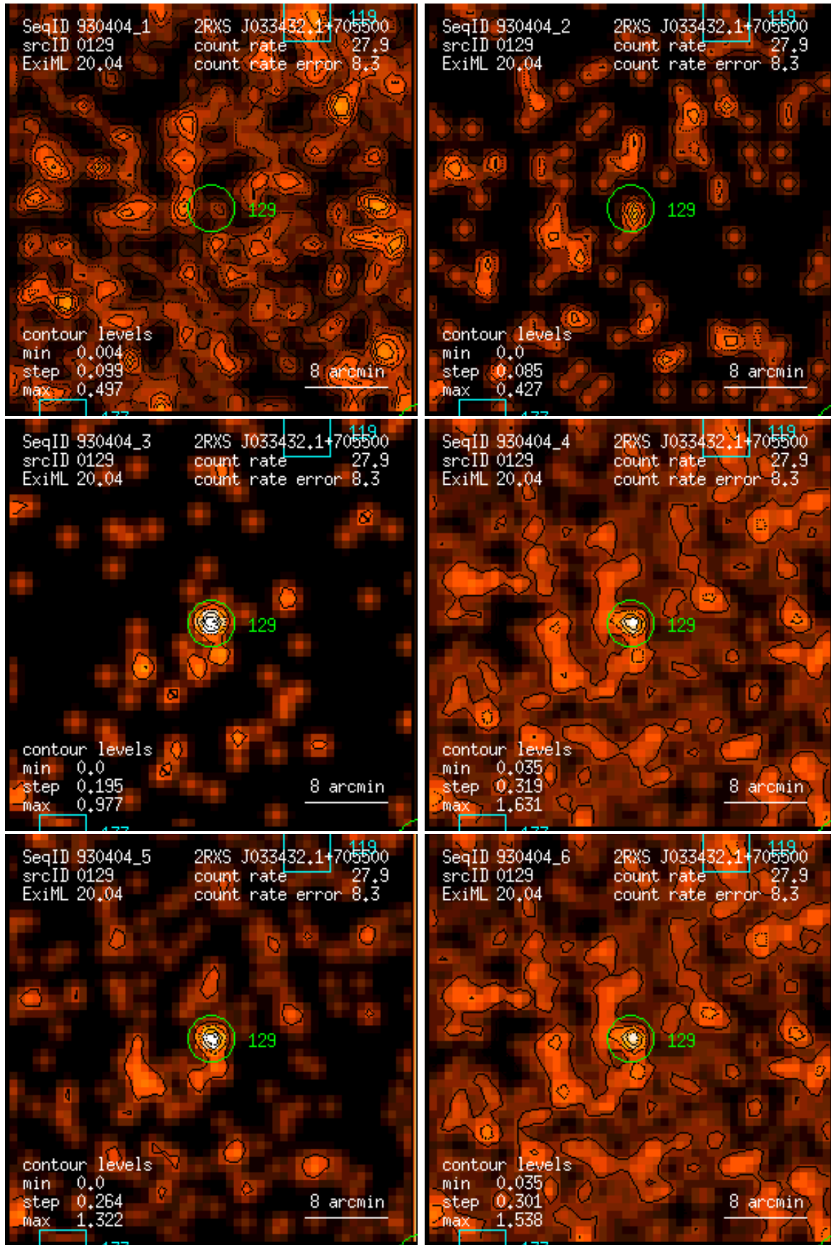
Figure 129: RASS 930404: detection 0129: band rate images, Gaussian filter: (1) PSPC channels 11 – 41, (2) 52 – 90, (3) 91 – 201, (4) 11 – 235, (5) 52 – 201, (6) 11 – 201. Broad band rates in counts/ks. Band rate contour levels in counts/ks/arcmin 2 .
