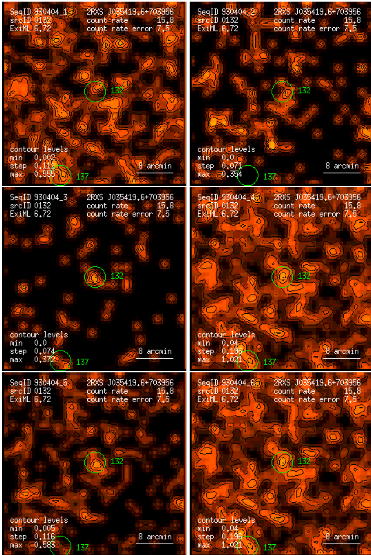
Figure 132: RASS 930404: detection 0132: band rate images, Gaussian filter: (1) PSPC channels 11 – 41, (2) 52 – 90, (3) 91 – 201, (4) 11 – 235, (5) 52 – 201, (6) 11 – 201. Broad band rates in counts/ks. Band rate contour levels in counts/ks/arcmin 2 .
