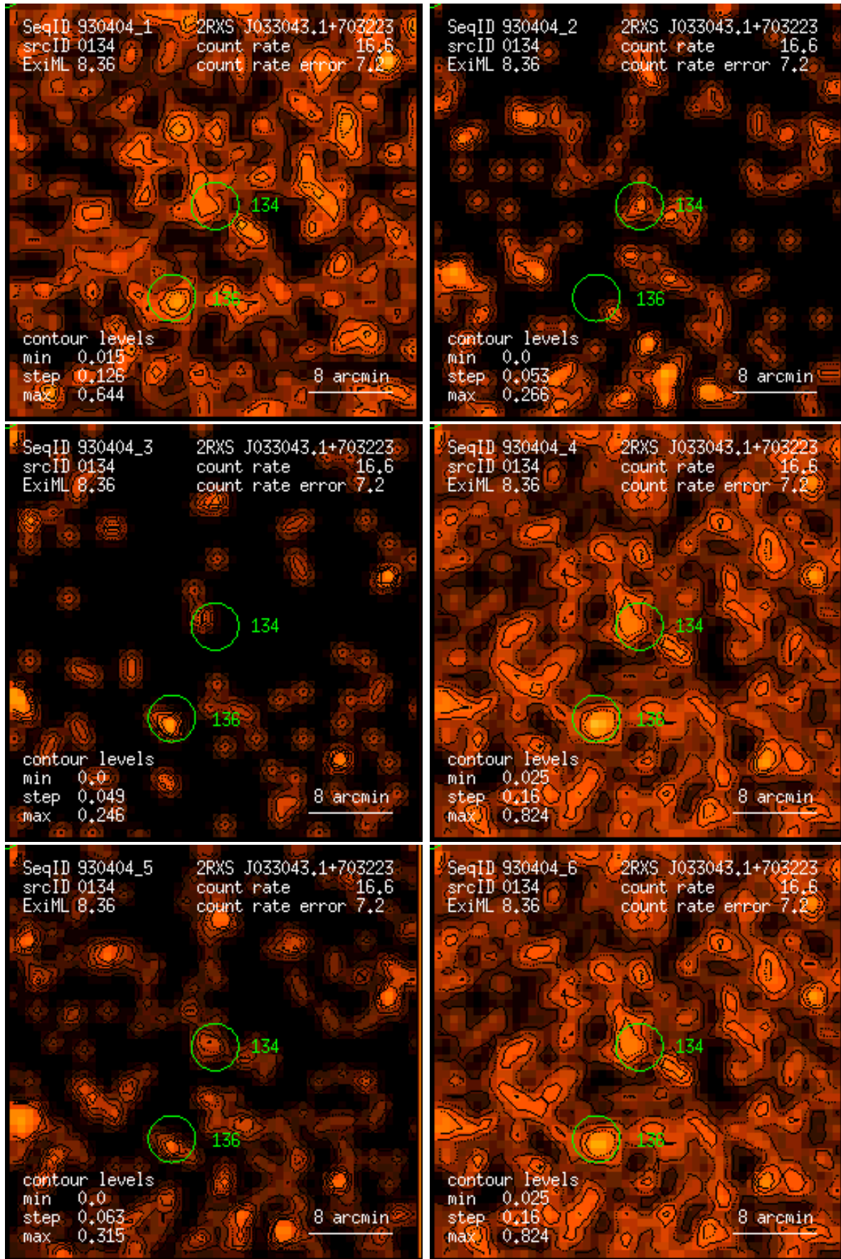
Figure 134: RASS 930404: detection 0134: band rate images, Gaussian filter: (1) PSPC channels 11 – 41, (2) 52 – 90, (3) 91 – 201, (4) 11 – 235, (5) 52 – 201, (6) 11 – 201. Broad band rates in counts/ks. Band rate contour levels in counts/ks/arcmin 2 .
