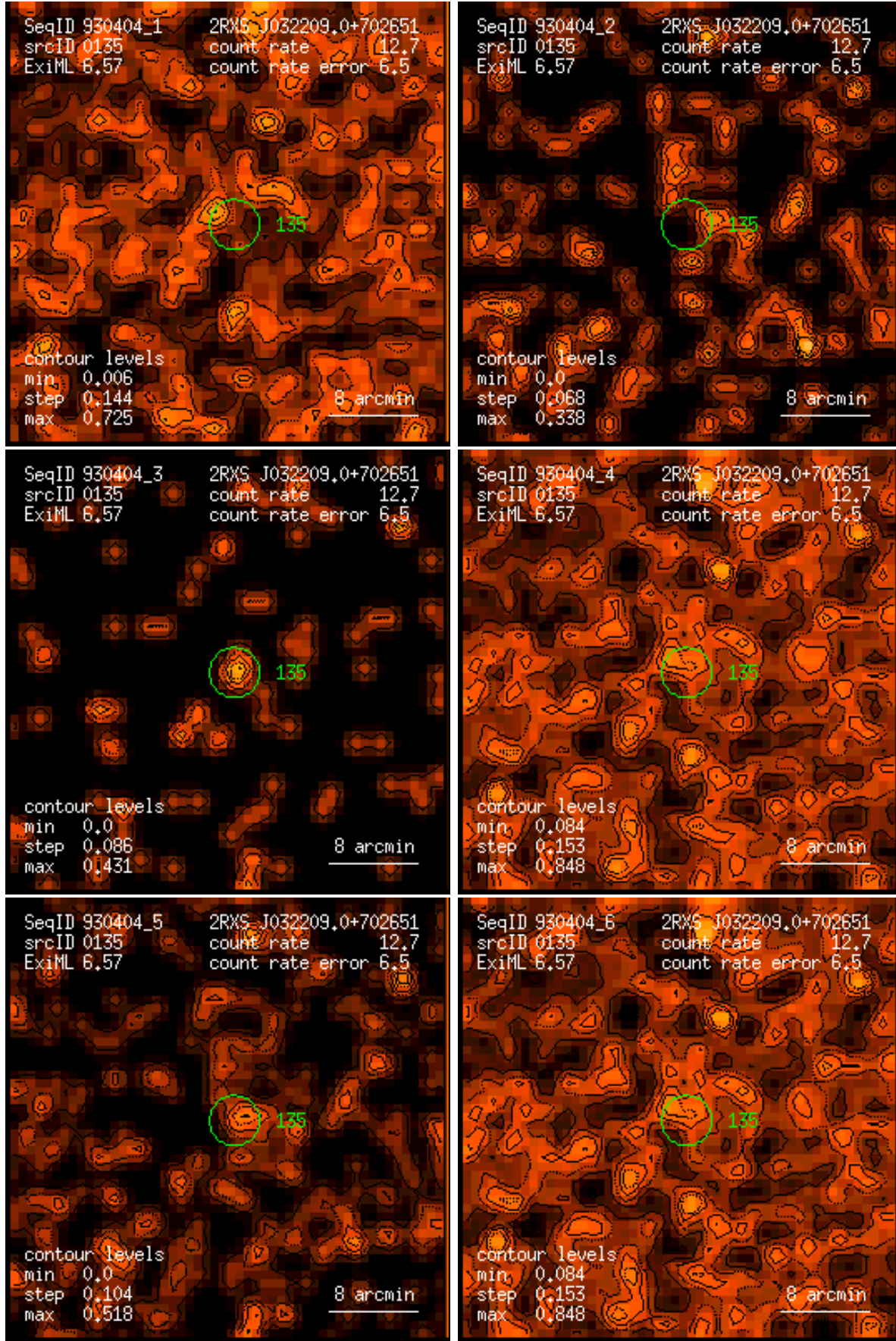
Figure 135: RASS 930404: detection 0135: band rate images, Gaussian filter: (1) PSPC channels 11 – 41, (2) 52 – 90, (3) 91 – 201, (4) 11 – 235, (5) 52 – 201, (6) 11 – 201. Broad band rates in counts/ks. Band rate contour levels in counts/ks/arcmin 2 .
