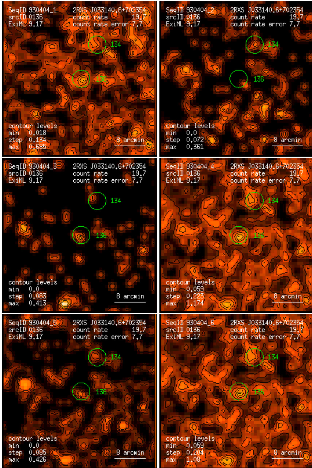
Figure 136: RASS 930404: detection 0136: band rate images, Gaussian filter: (1) PSPC channels 11 – 41, (2) 52 – 90, (3) 91 – 201, (4) 11 – 235, (5) 52 – 201, (6) 11 – 201. Broad band rates in counts/ks. Band rate contour levels in counts/ks/arcmin 2 .
