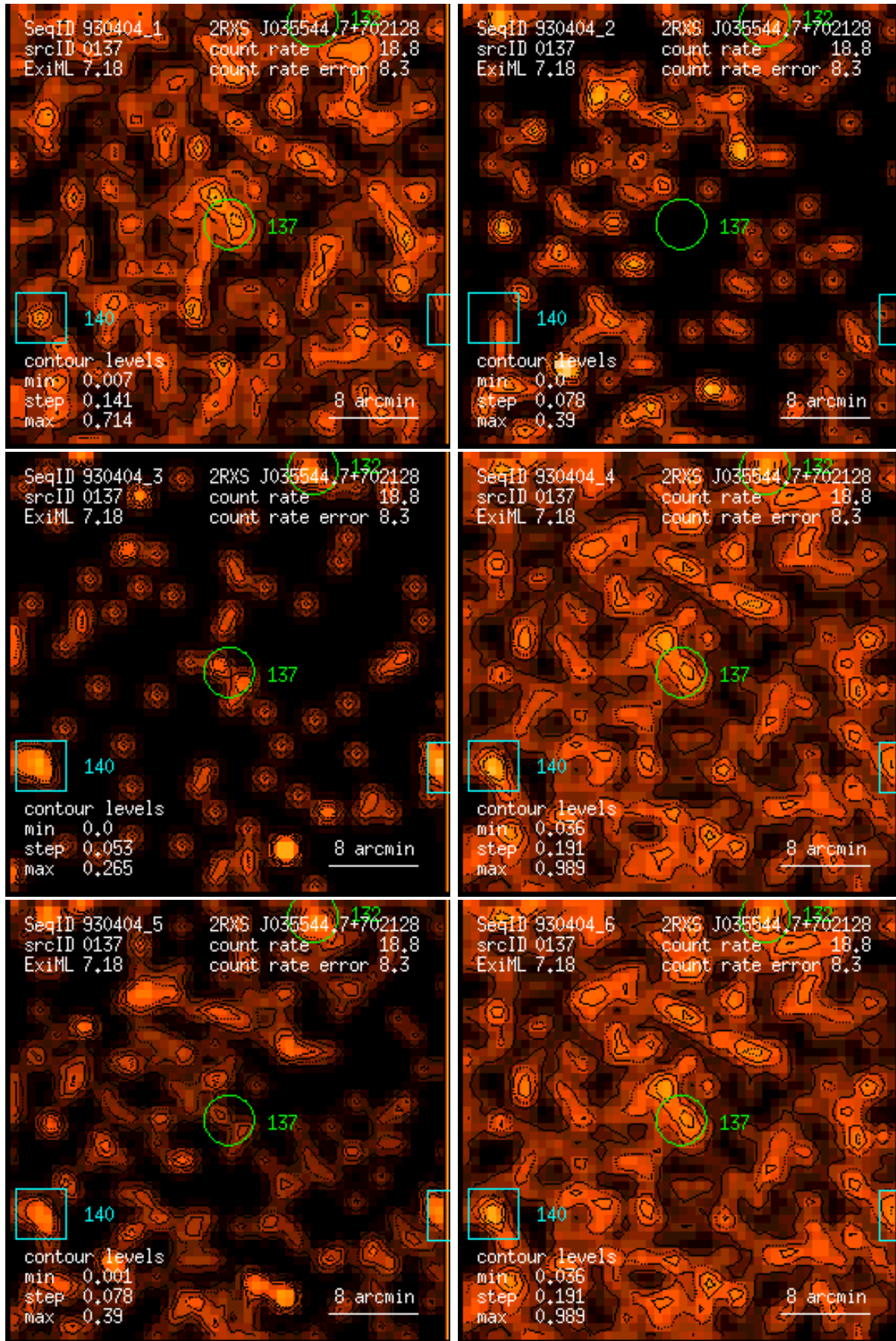
Figure 137: RASS 930404: detection 0137: band rate images, Gaussian filter: (1) PSPC channels 11 – 41, (2) 52 – 90, (3) 91 – 201, (4) 11 – 235, (5) 52 – 201, (6) 11 – 201. Broad band rates in counts/ks. Band rate contour levels in counts/ks/arcmin 2 .
