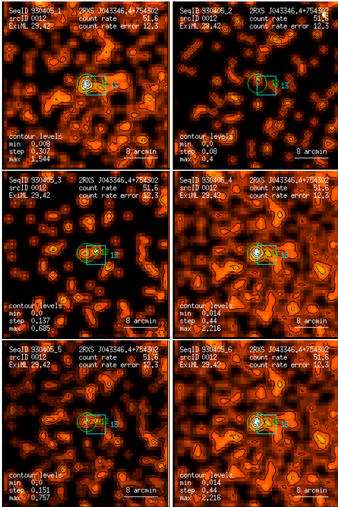
Figure 12: RASS 930405: detection 0012: band rate images, Gaussian filter: (1) PSPC channels 11 – 41, (2) 52 – 90, (3) 91 – 201, (4) 11 – 235, (5) 52 – 201, (6) 11 – 201. Broad band rates in counts/ks. Band rate contour levels in counts/ks/arcmin 2 .
