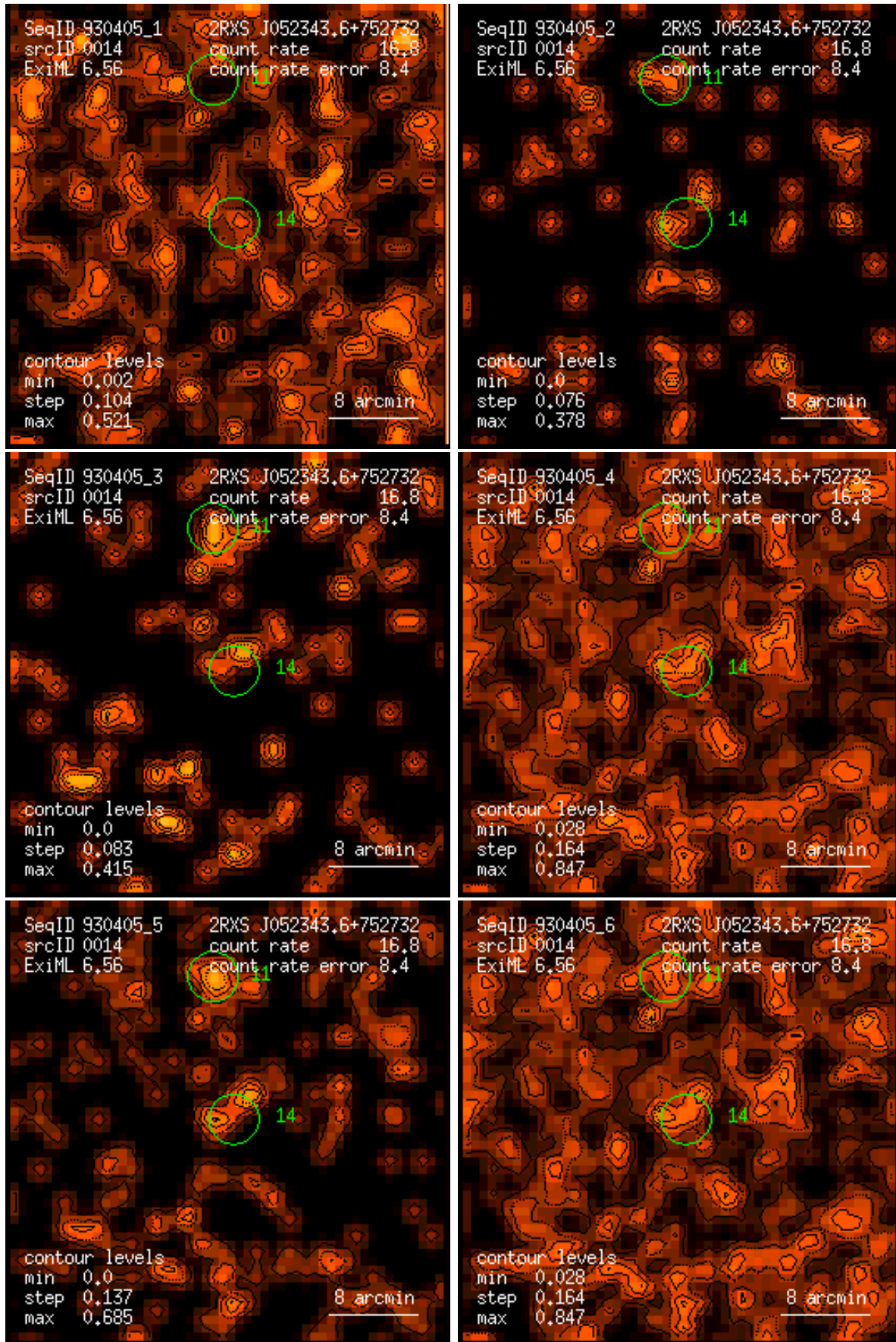
Figure 14: RASS 930405: detection 0014: band rate images, Gaussian filter: (1) PSPC channels 11 – 41, (2) 52 – 90, (3) 91 – 201, (4) 11 – 235, (5) 52 – 201, (6) 11 – 201. Broad band rates in counts/ks. Band rate contour levels in counts/ks/arcmin 2 .
