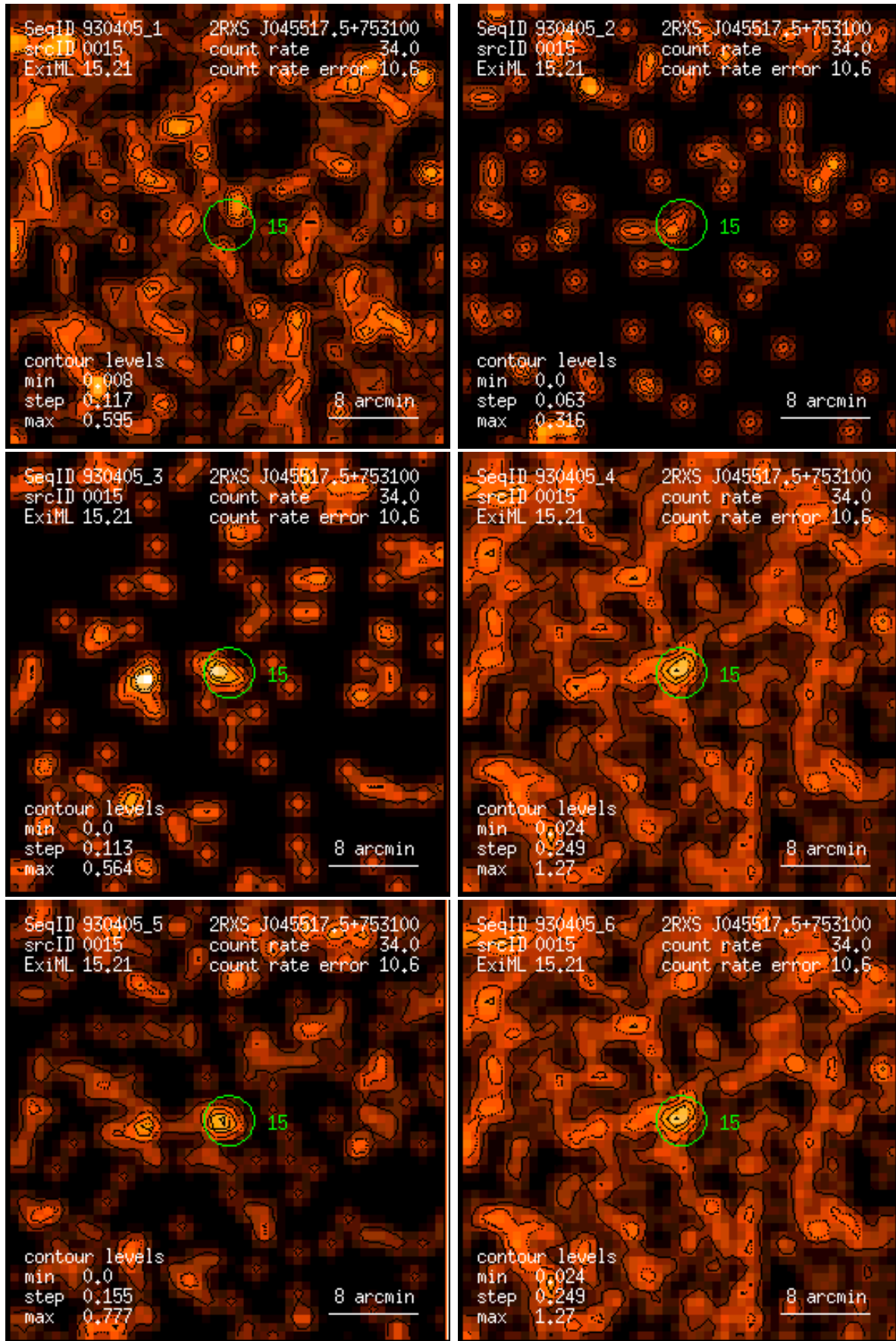
Figure 15: RASS 930405: detection 0015: band rate images, Gaussian filter: (1) PSPC channels 11 – 41, (2) 52 – 90, (3) 91 – 201, (4) 11 – 235, (5) 52 – 201, (6) 11 – 201. Broad band rates in counts/ks. Band rate contour levels in counts/ks/arcmin 2 .
