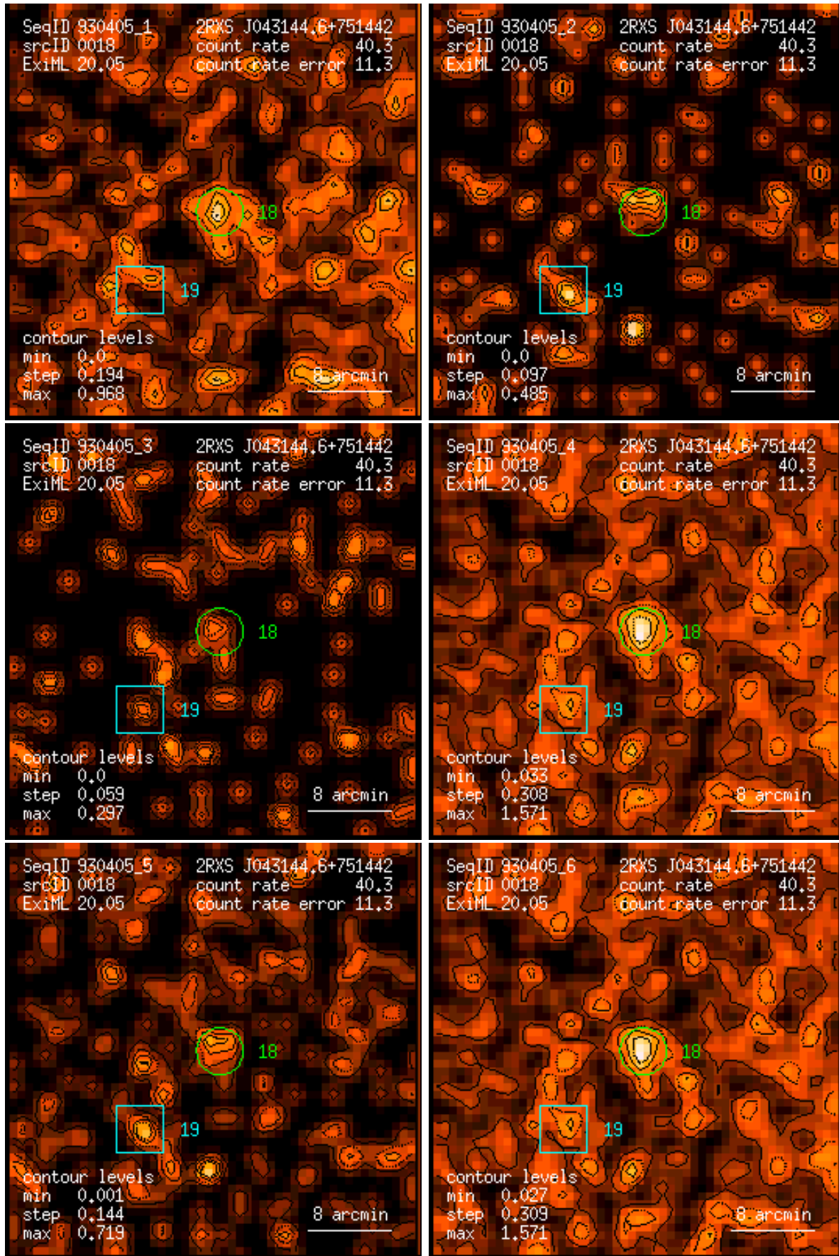
Figure 18: RASS 930405: detection 0018: band rate images, Gaussian filter: (1) PSPC channels 11 – 41, (2) 52 – 90, (3) 91 – 201, (4) 11 – 235, (5) 52 – 201, (6) 11 – 201. Broad band rates in counts/ks. Band rate contour levels in counts/ks/arcmin 2 .
