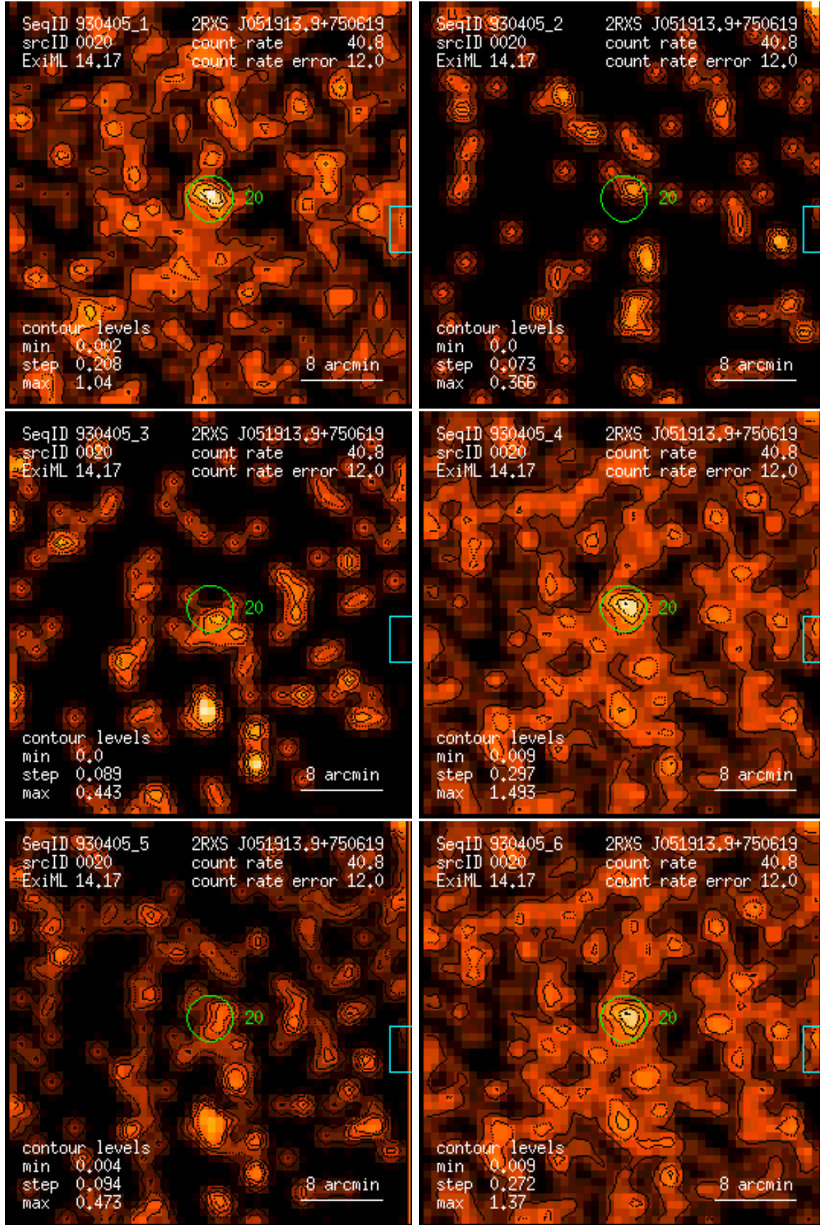
Figure 20: RASS 930405: detection 0020: band rate images, Gaussian filter: (1) PSPC channels 11 – 41, (2) 52 – 90, (3) 91 – 201, (4) 11 – 235, (5) 52 – 201, (6) 11 – 201. Broad band rates in counts/ks. Band rate contour levels in counts/ks/arcmin 2 .
