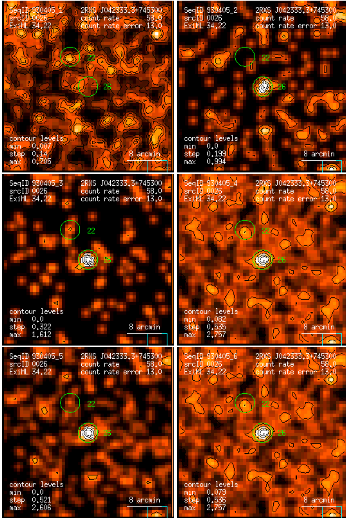
Figure 26: RASS 930405: detection 0026: band rate images, Gaussian filter: (1) PSPC channels 11 – 41, (2) 52 – 90, (3) 91 – 201, (4) 11 – 235, (5) 52 – 201, (6) 11 – 201. Broad band rates in counts/ks. Band rate contour levels in counts/ks/arcmin 2 .
