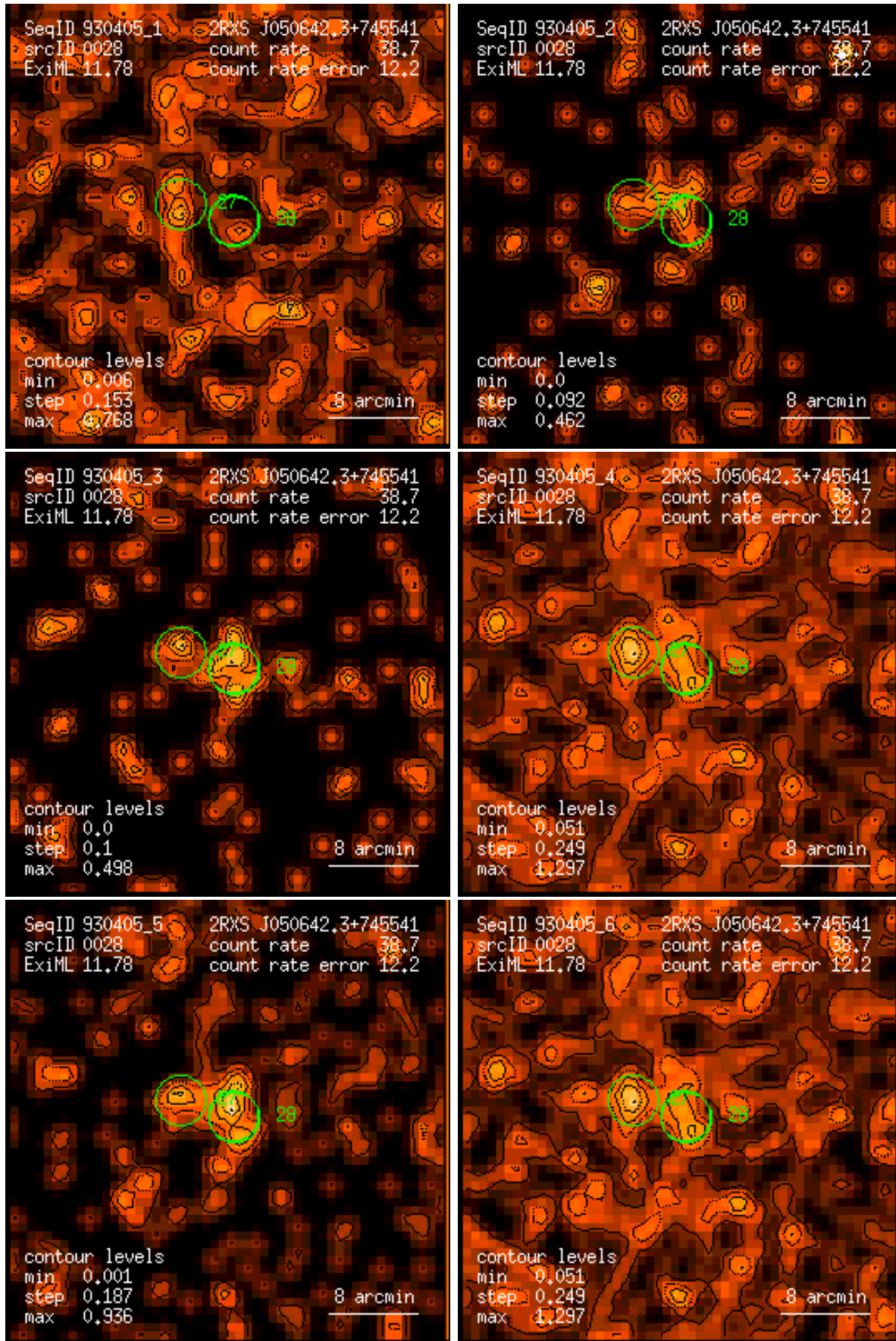
Figure 28: RASS 930405: detection 0028: band rate images, Gaussian filter: (1) PSPC channels 11 – 41, (2) 52 – 90, (3) 91 – 201, (4) 11 – 235, (5) 52 – 201, (6) 11 – 201. Broad band rates in counts/ks. Band rate contour levels in counts/ks/arcmin 2 .
