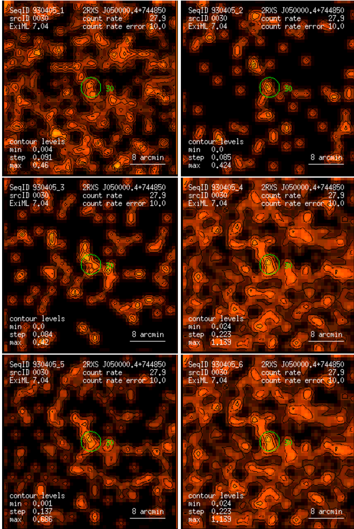
Figure 30: RASS 930405: detection 0030: band rate images, Gaussian filter: (1) PSPC channels 11 – 41, (2) 52 – 90, (3) 91 – 201, (4) 11 – 235, (5) 52 – 201, (6) 11 – 201. Broad band rates in counts/ks. Band rate contour levels in counts/ks/arcmin 2 .
