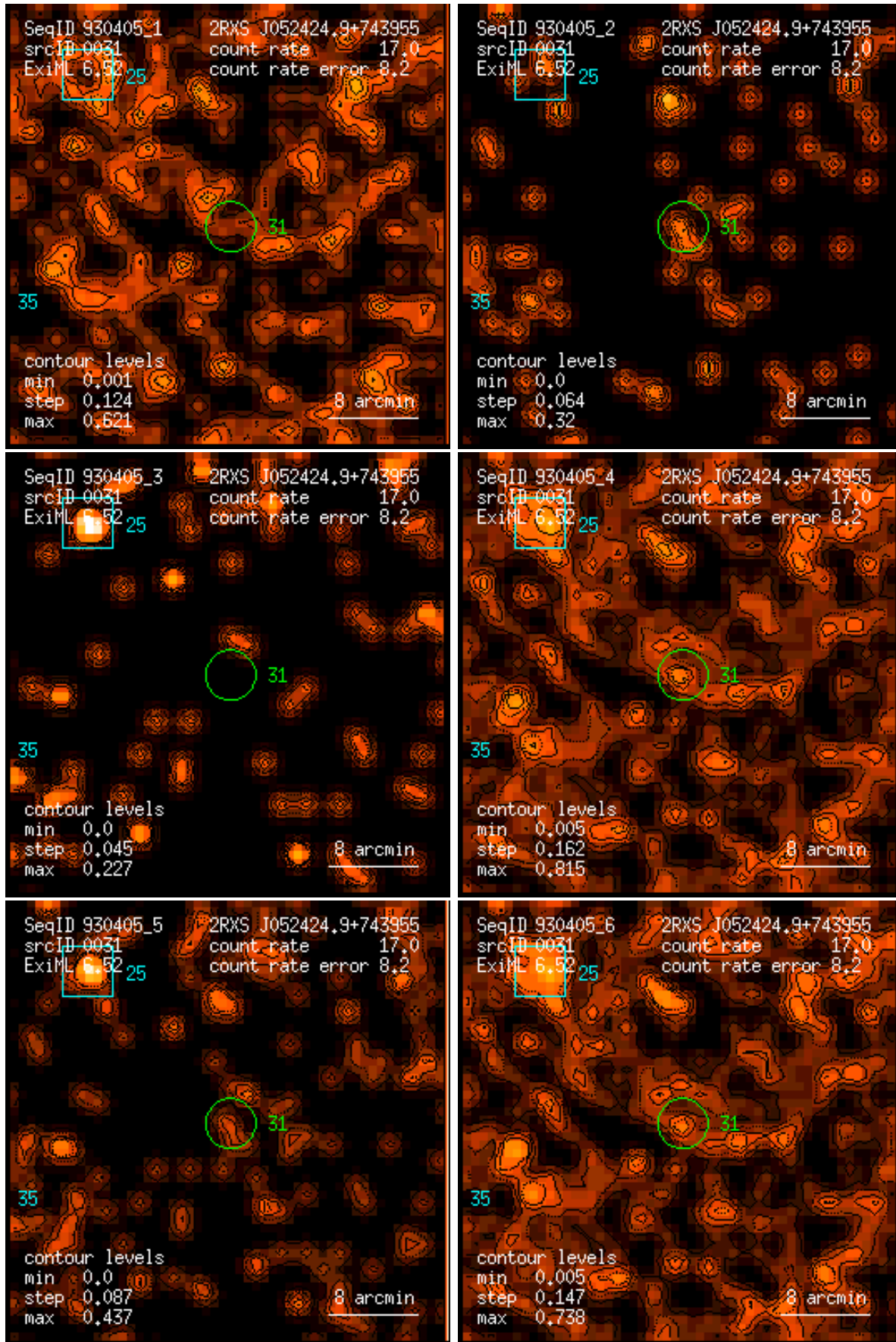
Figure 31: RASS 930405: detection 0031: band rate images, Gaussian filter: (1) PSPC channels 11 – 41, (2) 52 – 90, (3) 91 – 201, (4) 11 – 235, (5) 52 – 201, (6) 11 – 201. Broad band rates in counts/ks. Band rate contour levels in counts/ks/arcmin 2 .
