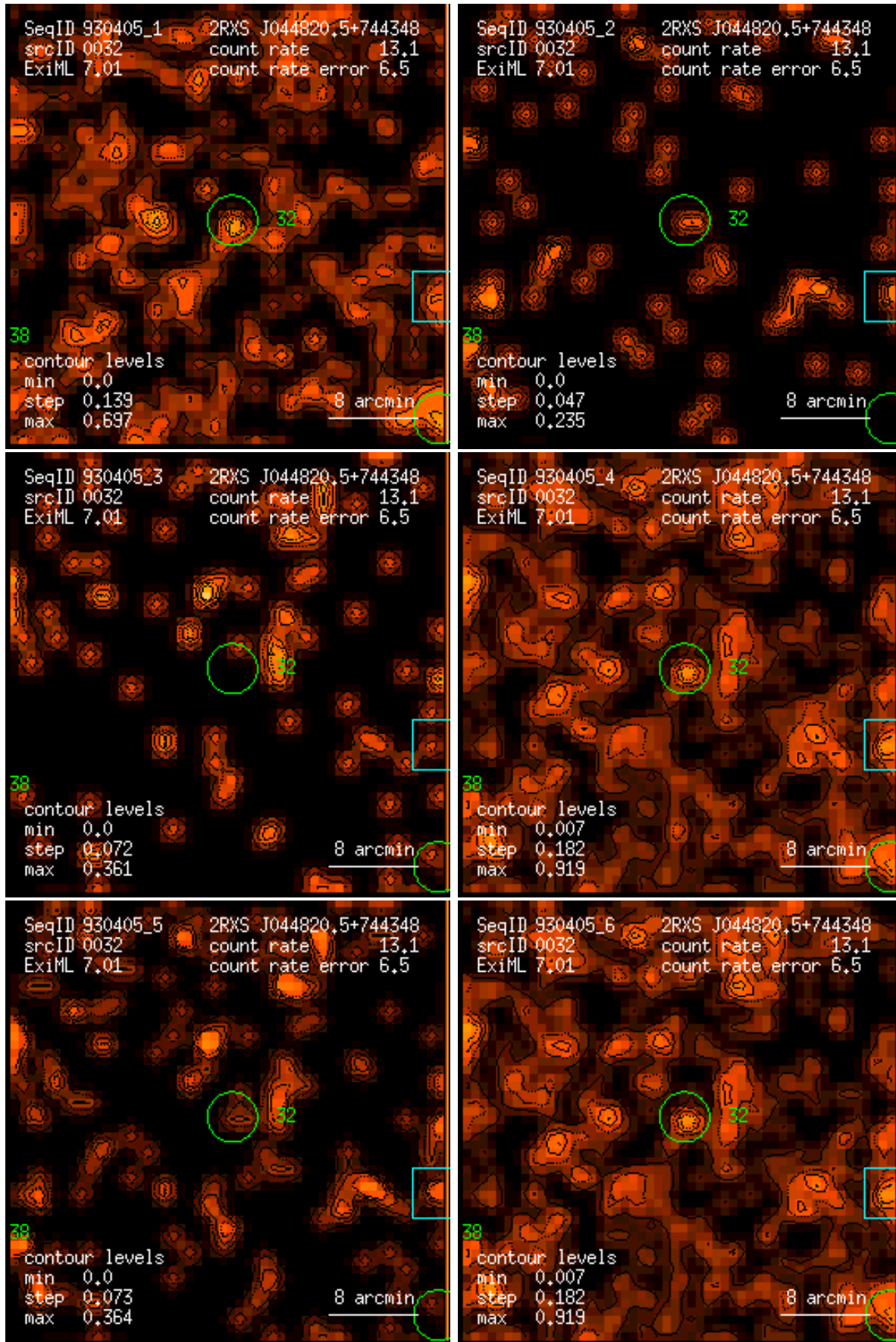
Figure 32: RASS 930405: detection 0032: band rate images, Gaussian filter: (1) PSPC channels 11 – 41, (2) 52 – 90, (3) 91 – 201, (4) 11 – 235, (5) 52 – 201, (6) 11 – 201. Broad band rates in counts/ks. Band rate contour levels in counts/ks/arcmin 2 .
