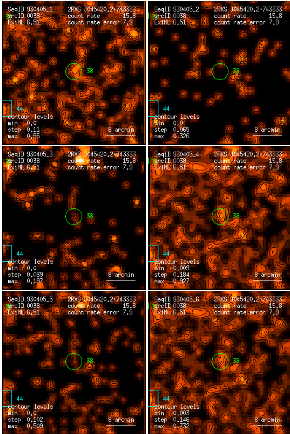
Figure 38: RASS 930405: detection 0038: band rate images, Gaussian filter: (1) PSPC channels 11 – 41, (2) 52 – 90, (3) 91 – 201, (4) 11 – 235, (5) 52 – 201, (6) 11 – 201. Broad band rates in counts/ks. Band rate contour levels in counts/ks/arcmin 2 .
