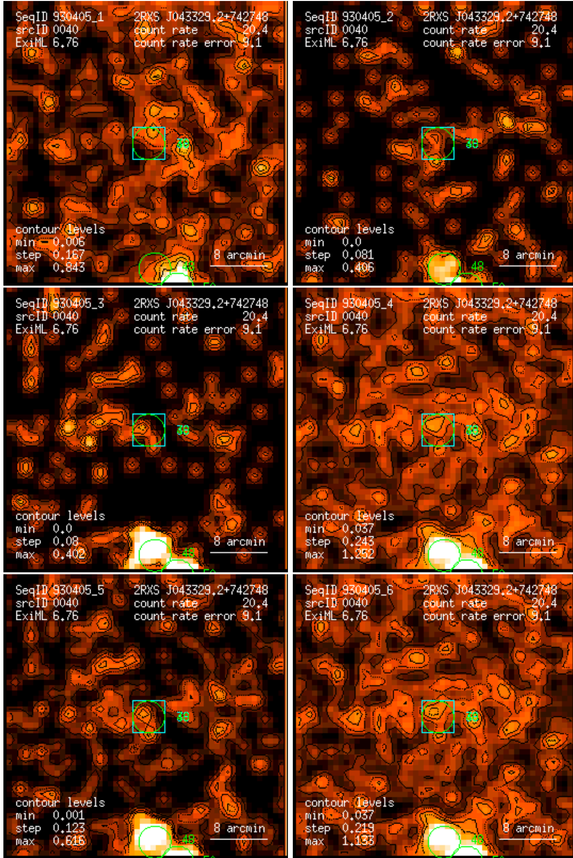
Figure 40: RASS 930405: detection 0040: band rate images, Gaussian filter: (1) PSPC channels 11 – 41, (2) 52 – 90, (3) 91 – 201, (4) 11 – 235, (5) 52 – 201, (6) 11 – 201. Broad band rates in counts/ks. Band rate contour levels in counts/ks/arcmin 2 .
