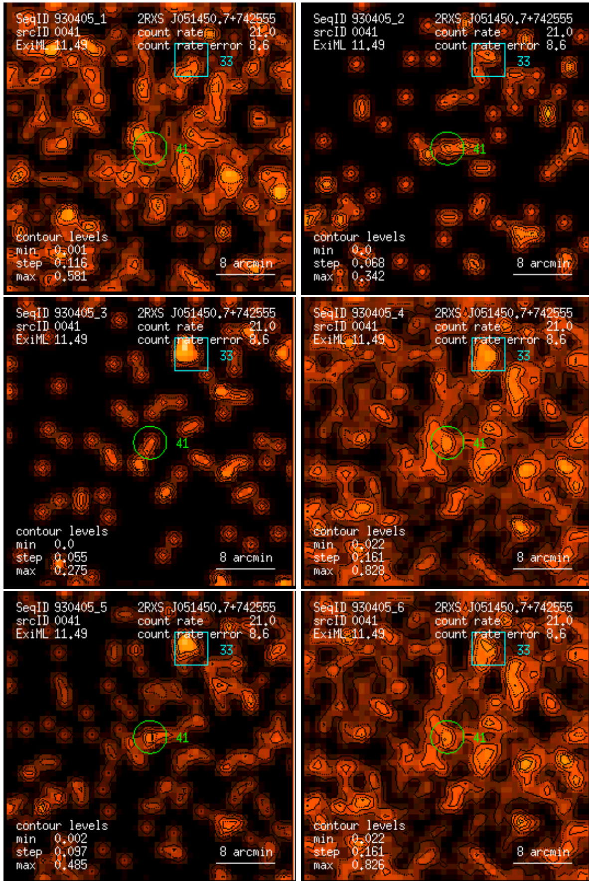
Figure 41: RASS 930405: detection 0041: band rate images, Gaussian filter: (1) PSPC channels 11 – 41, (2) 52 – 90, (3) 91 – 201, (4) 11 – 235, (5) 52 – 201, (6) 11 – 201. Broad band rates in counts/ks. Band rate contour levels in counts/ks/arcmin 2 .
