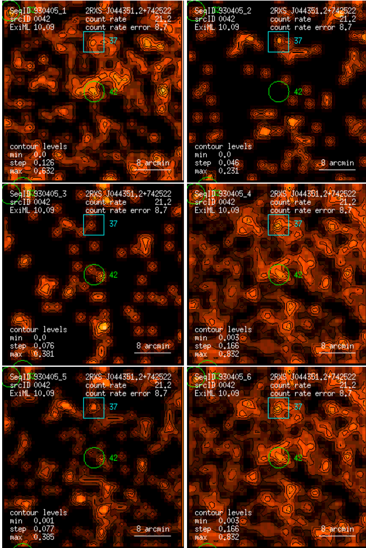
Figure 42: RASS 930405: detection 0042: band rate images, Gaussian filter: (1) PSPC channels 11 – 41, (2) 52 – 90, (3) 91 – 201, (4) 11 – 235, (5) 52 – 201, (6) 11 – 201. Broad band rates in counts/ks. Band rate contour levels in counts/ks/arcmin 2 .
