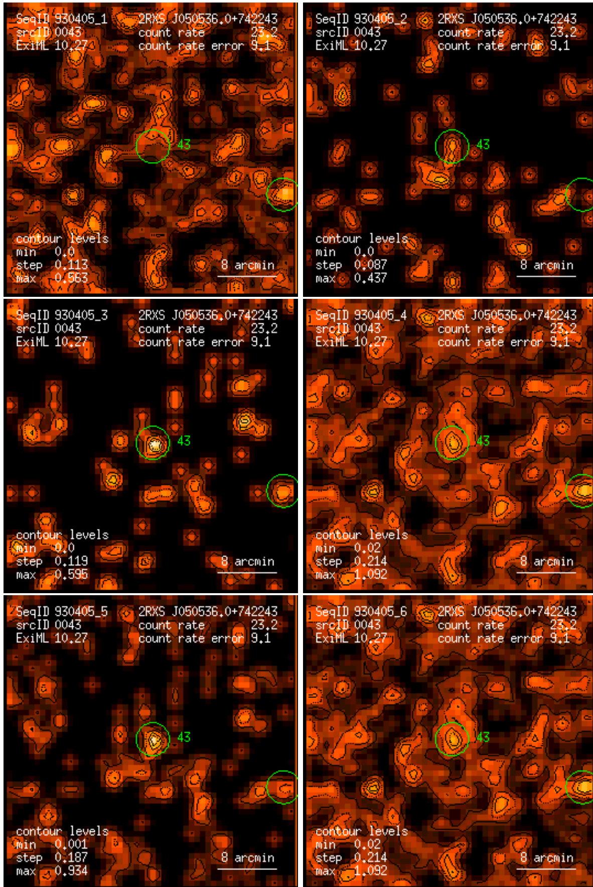
Figure 43: RASS 930405: detection 0043: band rate images, Gaussian filter: (1) PSPC channels 11 – 41, (2) 52 – 90, (3) 91 – 201, (4) 11 – 235, (5) 52 – 201, (6) 11 – 201. Broad band rates in counts/ks. Band rate contour levels in counts/ks/arcmin 2 .
