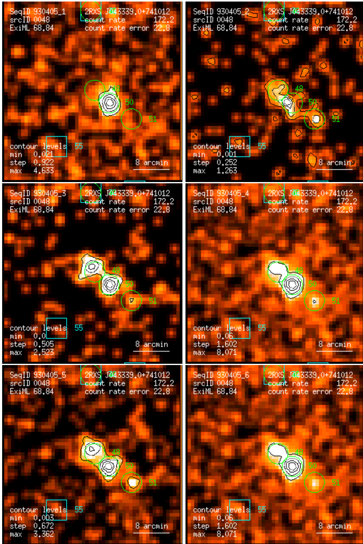
Figure 48: RASS 930405: detection 0048: band rate images, Gaussian filter: (1) PSPC channels 11 – 41, (2) 52 – 90, (3) 91 – 201, (4) 11 – 235, (5) 52 – 201, (6) 11 – 201. Broad band rates in counts/ks. Band rate contour levels in counts/ks/arcmin 2 .
