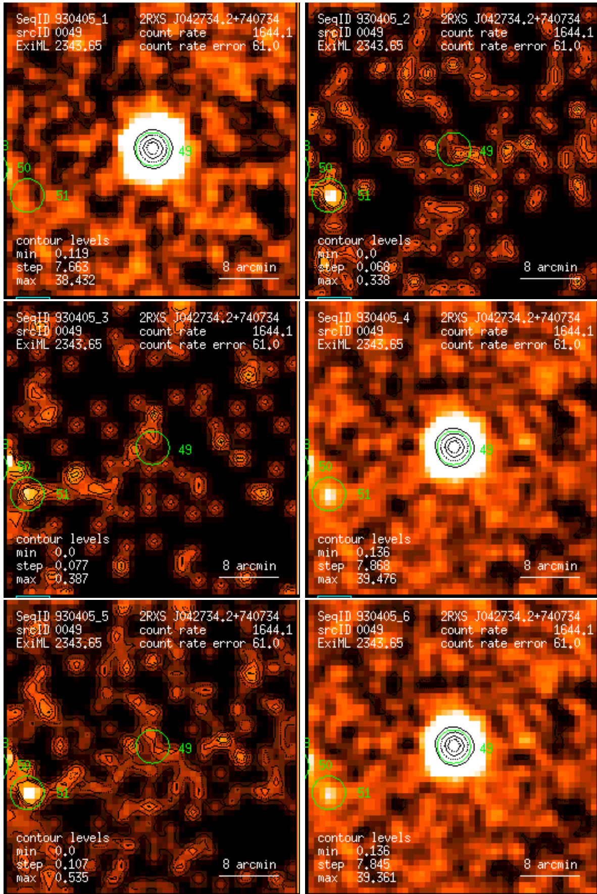
Figure 49: RASS 930405: detection 0049: band rate images, Gaussian filter: (1) PSPC channels 11 – 41, (2) 52 – 90, (3) 91 – 201, (4) 11 – 235, (5) 52 – 201, (6) 11 – 201. Broad band rates in counts/ks. Band rate contour levels in counts/ks/arcmin 2 .
