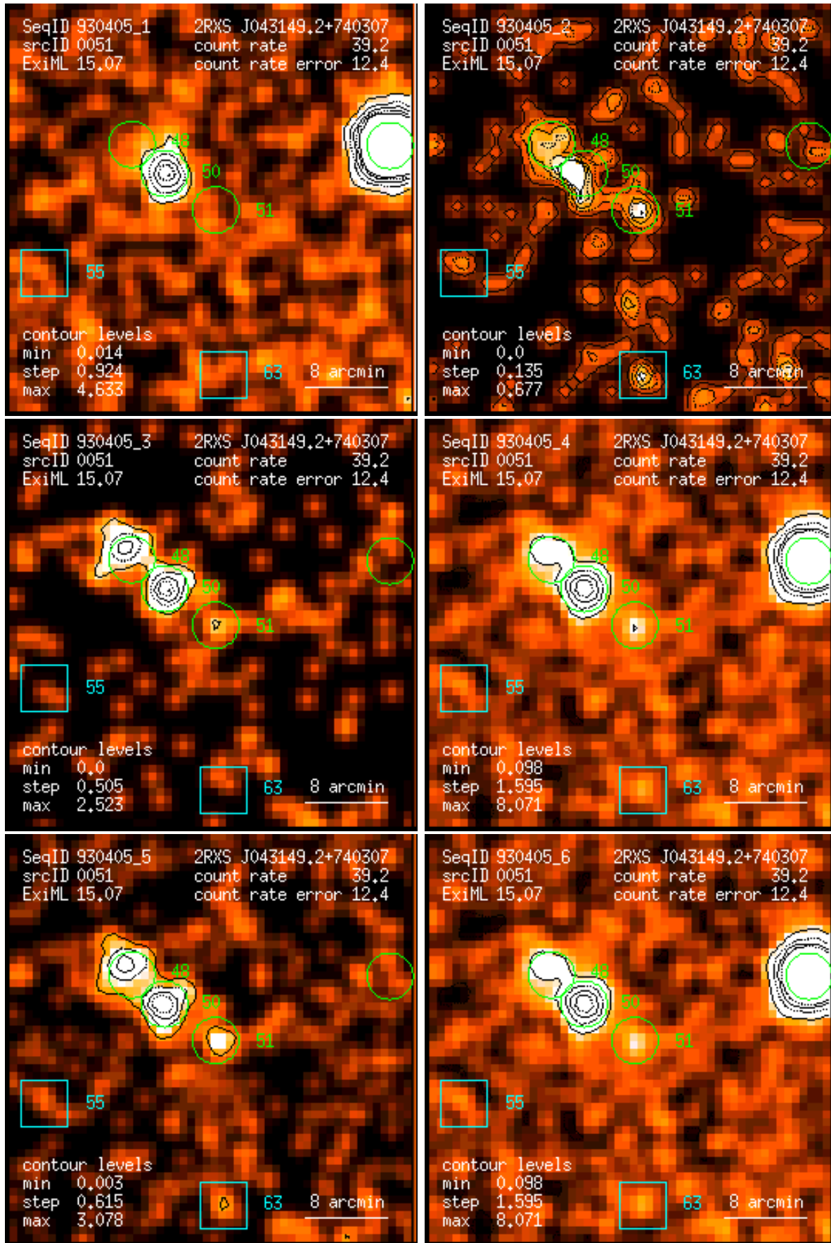
Figure 51: RASS 930405: detection 0051: band rate images, Gaussian filter: (1) PSPC channels 11 – 41, (2) 52 – 90, (3) 91 – 201, (4) 11 – 235, (5) 52 – 201, (6) 11 – 201. Broad band rates in counts/ks. Band rate contour levels in counts/ks/arcmin 2 .
