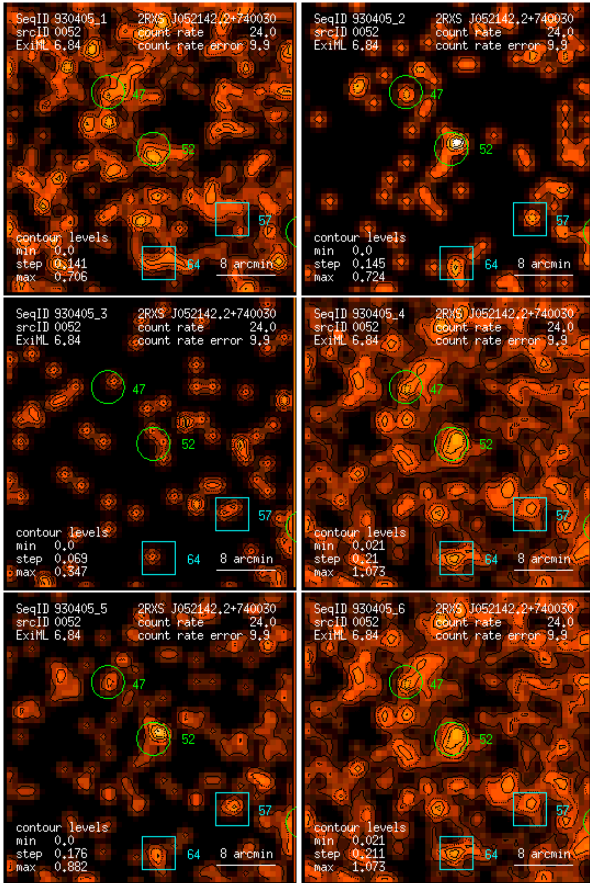
Figure 52: RASS 930405: detection 0052: band rate images, Gaussian filter: (1) PSPC channels 11 – 41, (2) 52 – 90, (3) 91 – 201, (4) 11 – 235, (5) 52 – 201, (6) 11 – 201. Broad band rates in counts/ks. Band rate contour levels in counts/ks/arcmin 2 .
